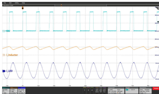
Figure 9-15. LED Current Ripple at PWM_{ADIM} = 100\% , 1 kHz and F_{SW} = 1.2 MHz
