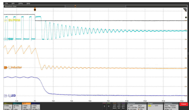
Figure 9-16. LED PWM Dimming at PWM_{PWM} = 90\% , 20 kHz
