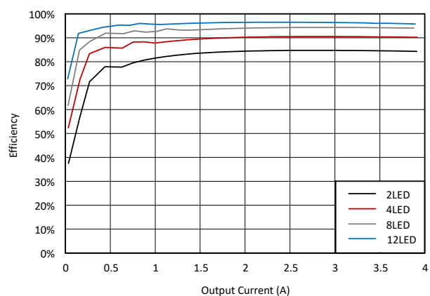
Figure 7-12. Efficiency at 48-V Input Voltage, 4-A Output Current
