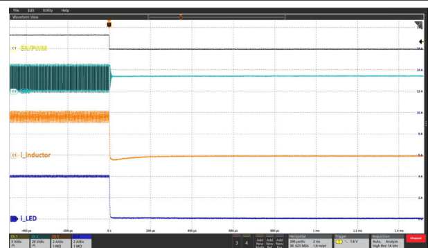
Figure 9-5. LED Current Transient for a PWM ADIM Transition from 99% to 1%, 1 kHz
