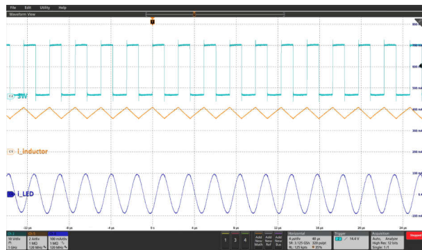
Figure 9-2. LED Current Ripple at PWM ADIM = 100%, 1 kHz and F SW = 400 kHz
