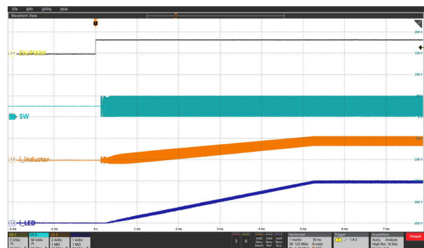
Figure 9-21. Start-Up at PWM PWM = 100%, 20 kHz
