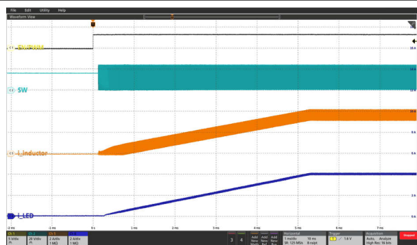
Figure 9-4. LED Current Transient for a PWM ADIM Transition from 1% to 99%, 1 kHz
