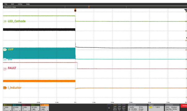
Figure 9-9. LED- Short-to-PGND Protection
