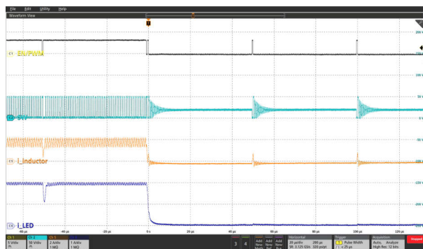
Figure 9-18. LED PWM Dimming Falling Edge at PWM_{PWM} = 50\% , 20 kHz
