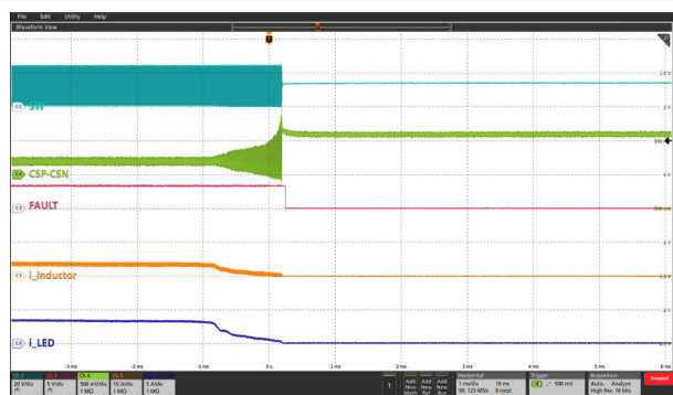
Figure 9-10. LED+ and LED- Short-Circuit Protection
