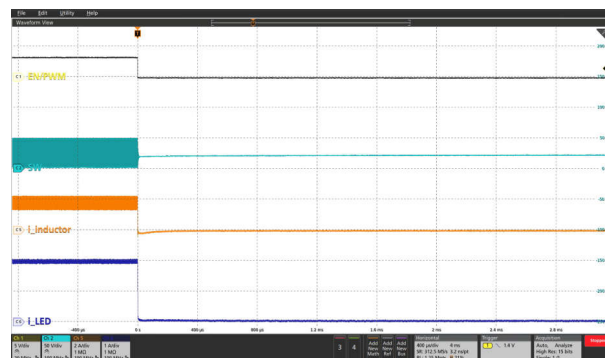
Figure 9-22. Shutdown at PWM PWM = 100%, 20 kHz
