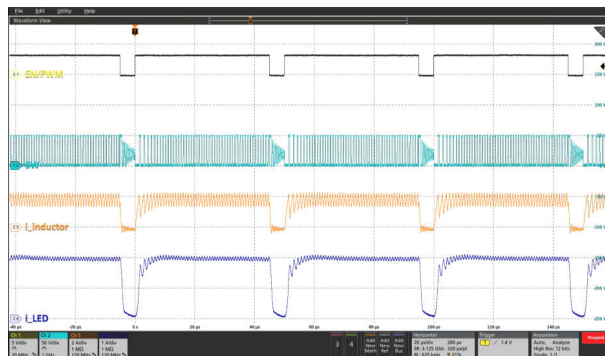
Figure 9-16. LED PWM Dimming at PWM_{PWM} = 90\% , 20 kHz
