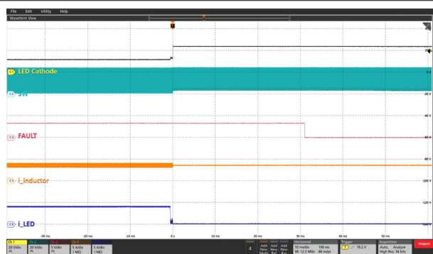
Figure 9-8. LED Open-Load Protection
