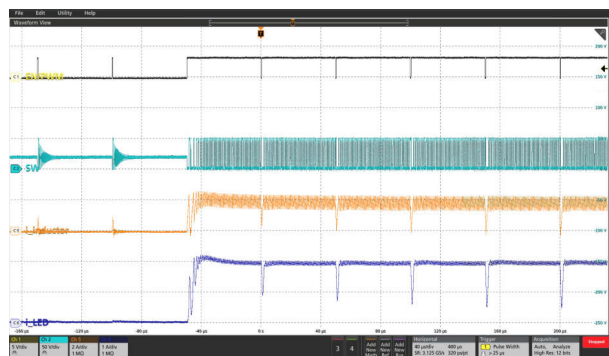
Figure 9-17. LED PWM Dimming Rising Edge at PWM_{PWM} = 50\% , 20 kHz
