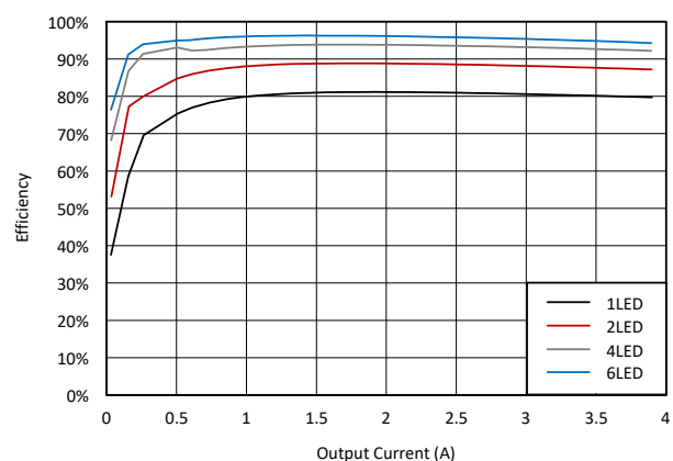
Figure 7-11. Efficiency at 24-V Input Voltage, 4-A Output Current
