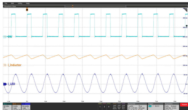
Figure 9-15. LED Current Ripple at PWM_{ADIM} = 100\% , 1 kHz and F_{SW} = 1.2 MHz
