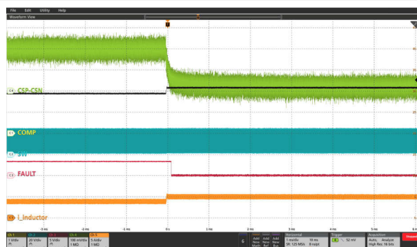
Figure 9-11. Switching FET Short-Circuit Protection
