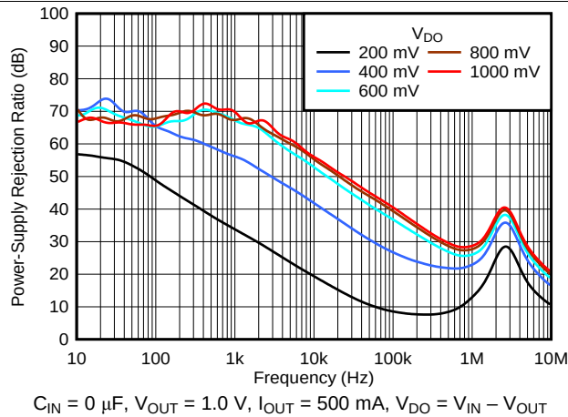
图 25. V_{IN} PSRR vs Frequency and Dropout
