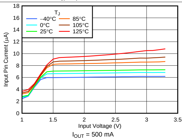
图 11. I_{Q(IN)} vs V_{IN} and Temperature
