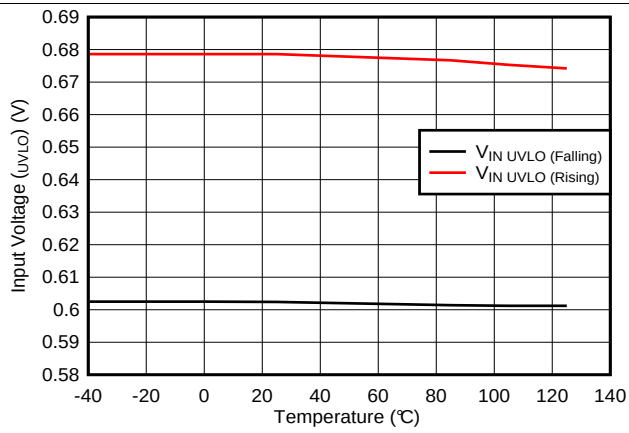
图 31. V_{UVLO(IN)} Rising and Falling Threshold vs Temperature
