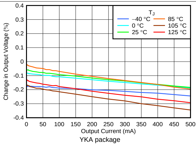
图 3. Output Accuracy vs I_{OUT} and Temperature
