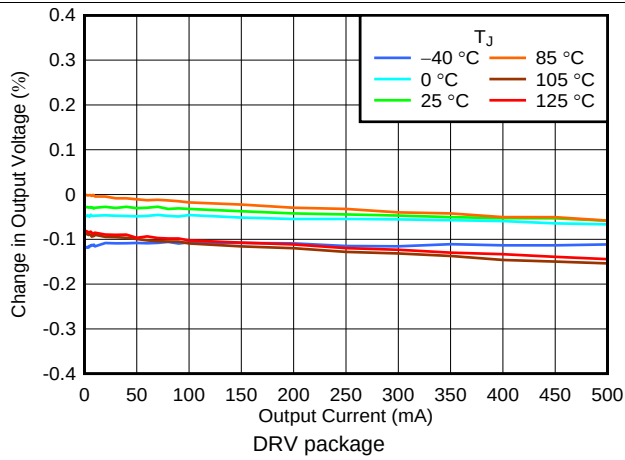
图 1. Output Accuracy vs I_{OUT} and Temperature
