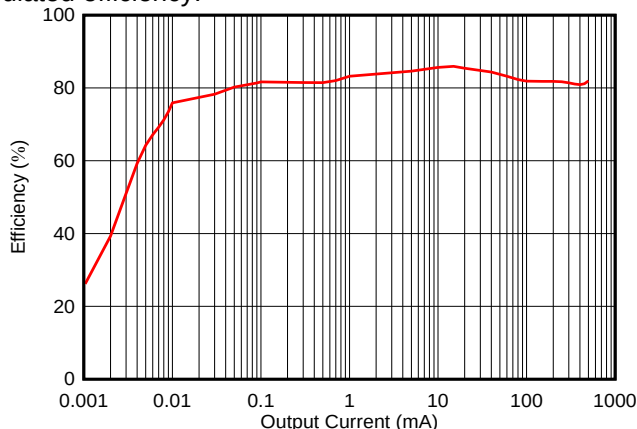
图 38. TPS7A11 Output Efficiency at 1.2 V_{IN} and 1.0 V_{OUT}
