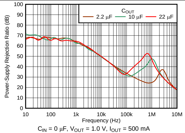
图 26. V_{IN} PSRR vs Frequency and C_{OUT}
