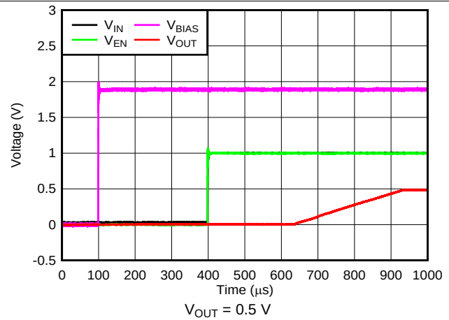
图 14. Startup With V_{EN} = V_{IN}
