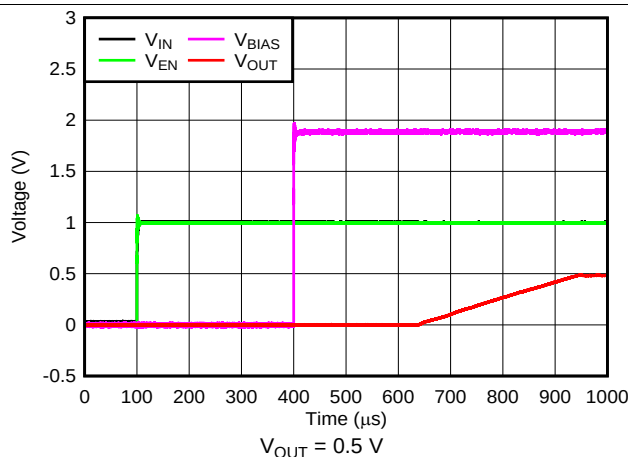
图 17. Startup With V_{BIAS} Powering Up After V_{IN} and V_{EN}
