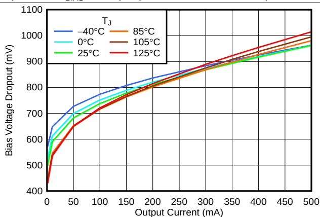
图 7. V_{BIAS} Dropout vs I_{OUT} and Temperature
