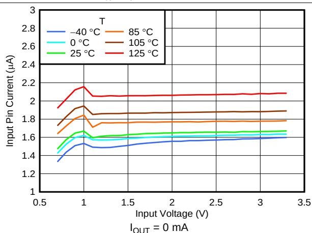
图 10. I_{Q(IN)} vs V_{IN} and Temperature
