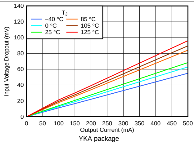
图 5. V_{IN} Dropout vs I_{OUT} and Temperature
