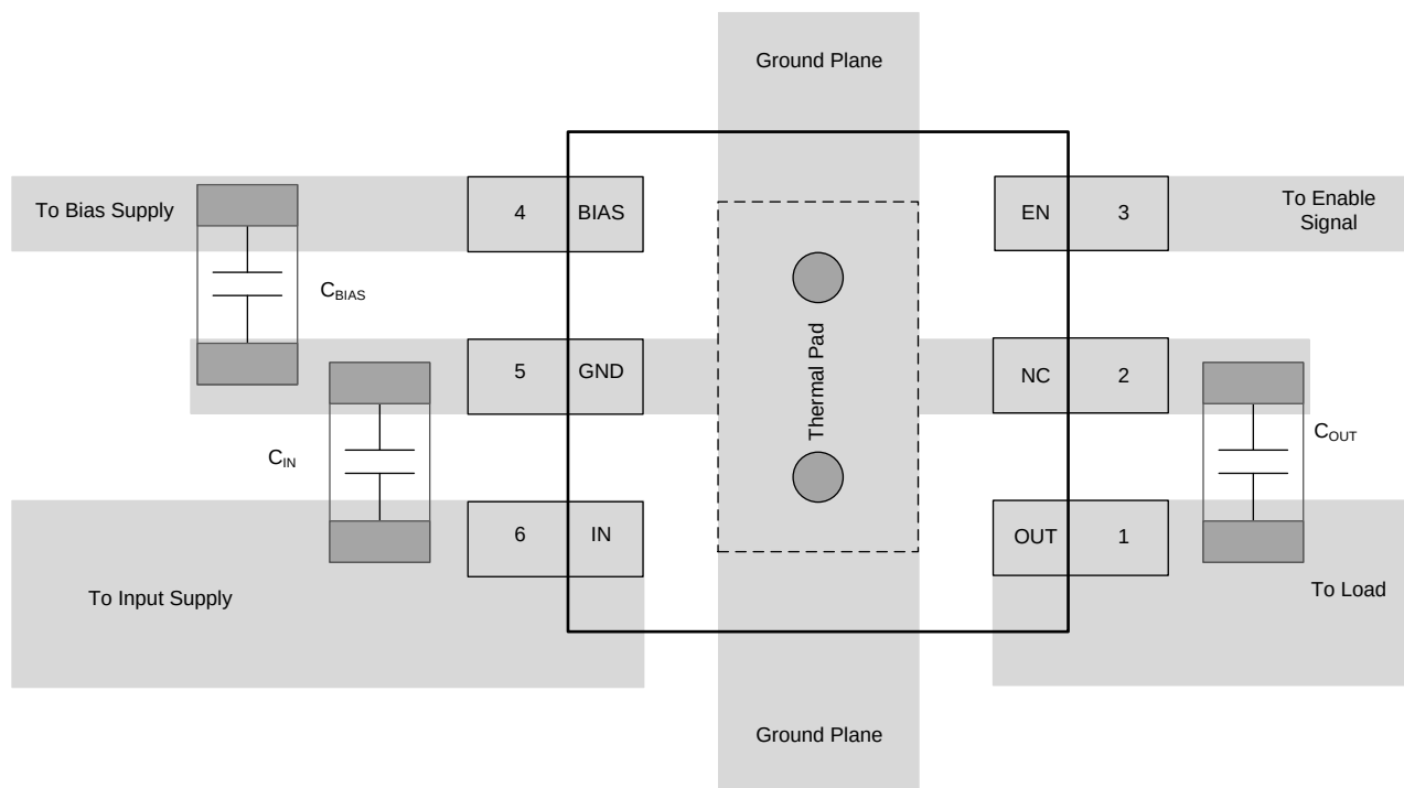
图 40. Recommended Layout for DRV Package
