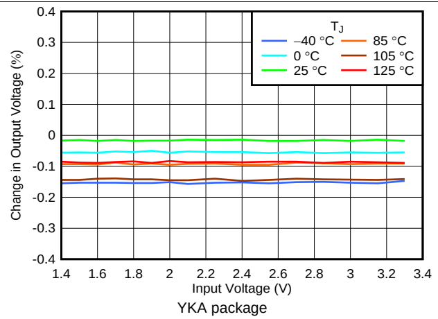
图 2. Output Accuracy vs V_{IN} and Temperature
