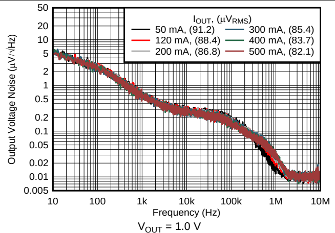
图 28. Output Noise vs Frequency and I_{OUT}
