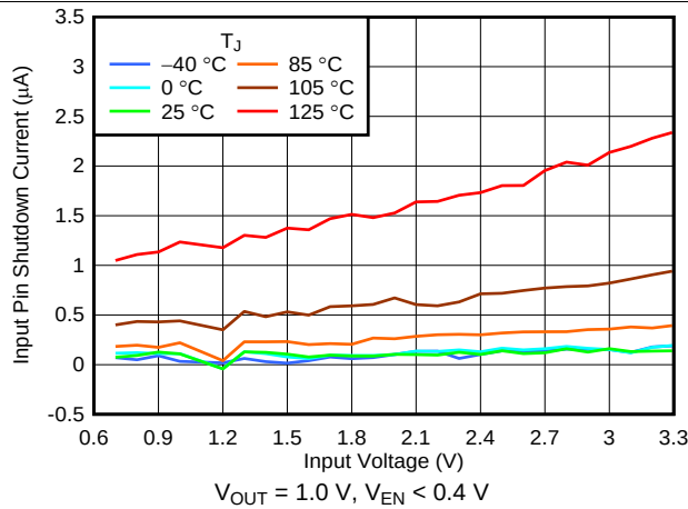
图 13. I_{SHDN} vs V_{IN} and Temperature
