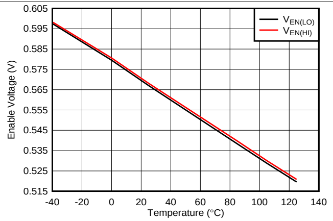
图 32. Enable High and Low Threshold vs Temperature
