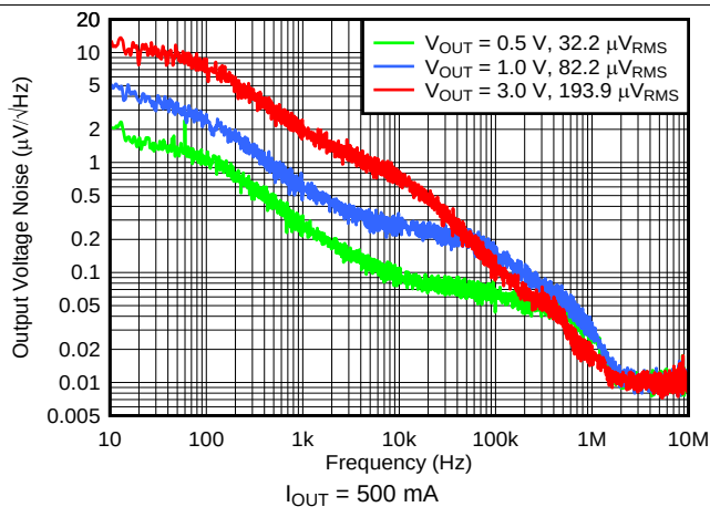
图 29. Output Noise vs Frequency and V_{OUT}
