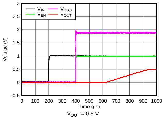
图 15. Startup With V_{EN} and V_{BIAS} Powering Up Simultaneously
