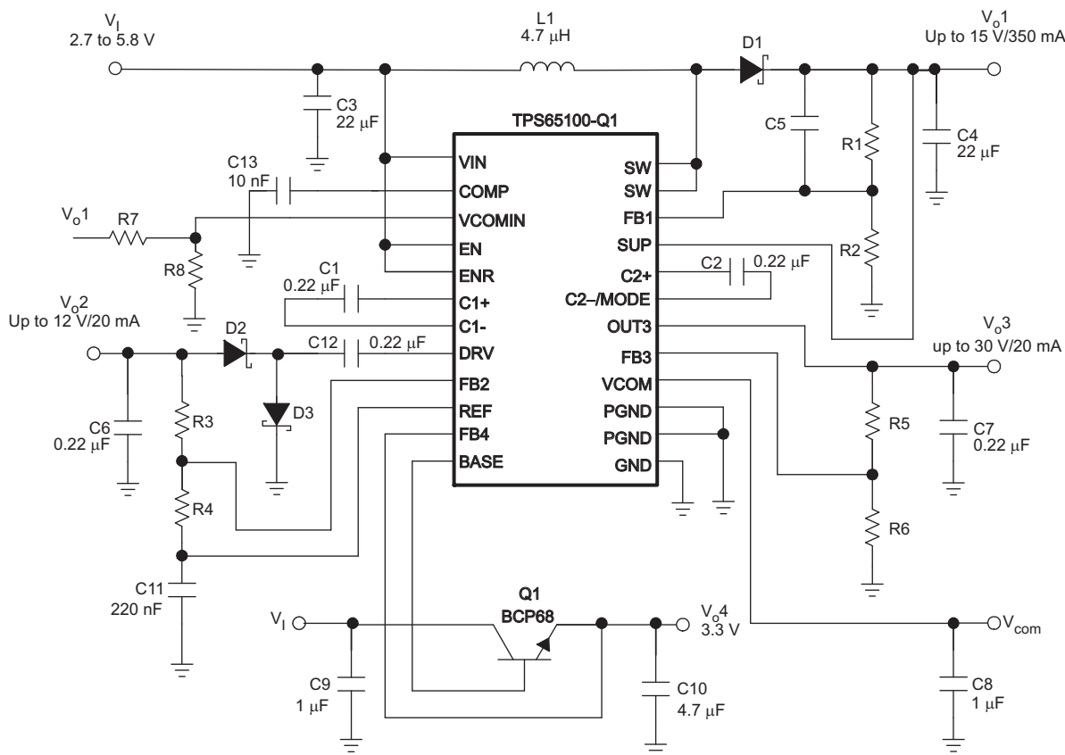
Figure 3. Simplified Schematic
