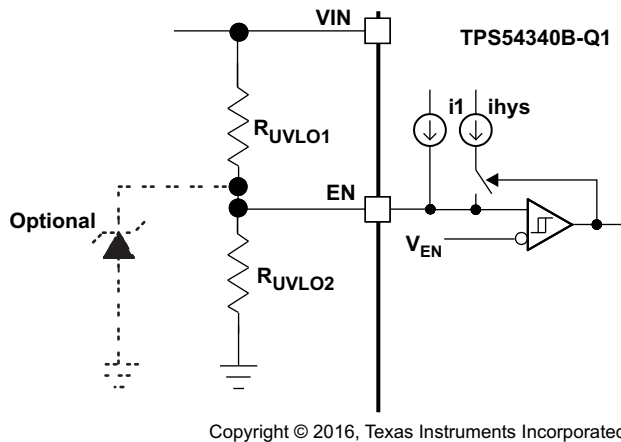
Figure 22. Adjustable Undervoltage Lockout (UVLO)
