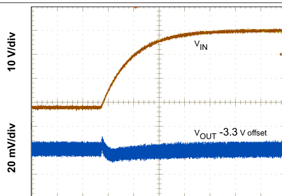
Figure 35. Line Transient (8 V to 40 V)
