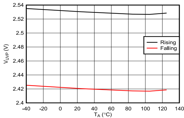
图 7-8. IN Undervoltage Threshold vs Temperature
