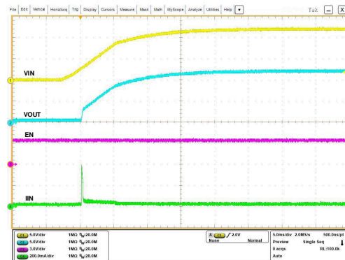
图 7-39. Start-Up with Supply
