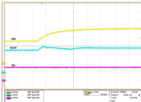
图 7-45. Overvoltage Lockout Response - TPS259470x/4x
