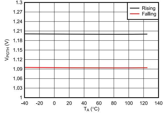
图 7-33. PGTH Threshold vs Temperature
