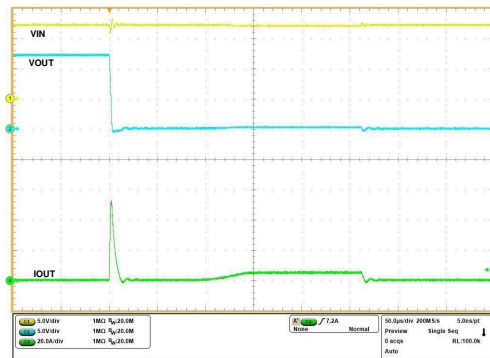
图 7-51. Transient Overcurrent Blanking Timer Response - TPS25947x
