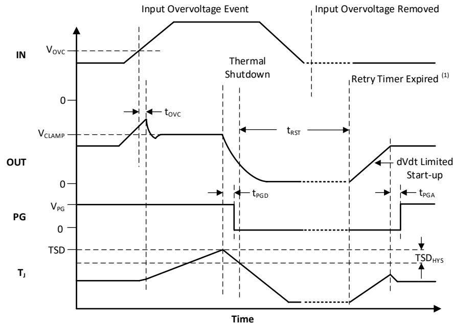
图 8-8. TPS25947x Overvoltage Response (Auto-Retry)
