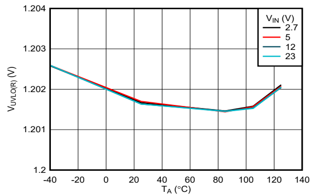
图 7-9. EN/UVLO Rising Threshold vs Temperature
