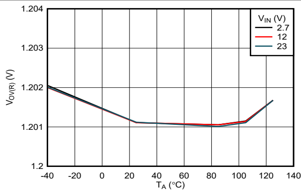
图 7-12. OVLO Rising Threshold vs Temperature
