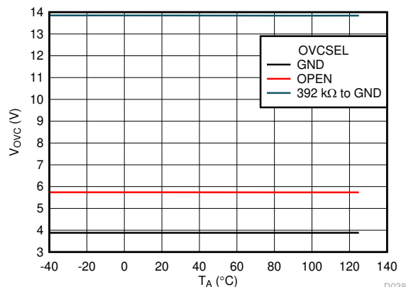
图 7-24. OVC Threshold vs Temperature
