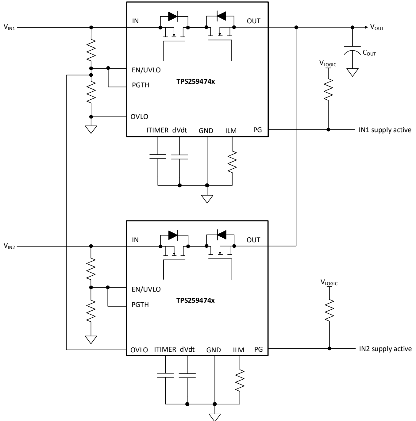
图 9-15. Priority power MUXing with 2 × TPS259474x
