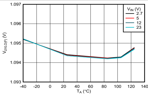
图 7-10. EN/UVLO Falling Threshold vs Temperature
