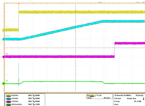
图 7-38. Start-Up with Enable
