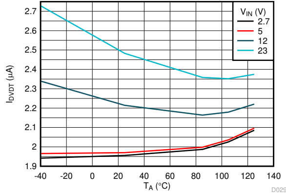
图 7-32. DVDVT Charging Current vs Temperature
