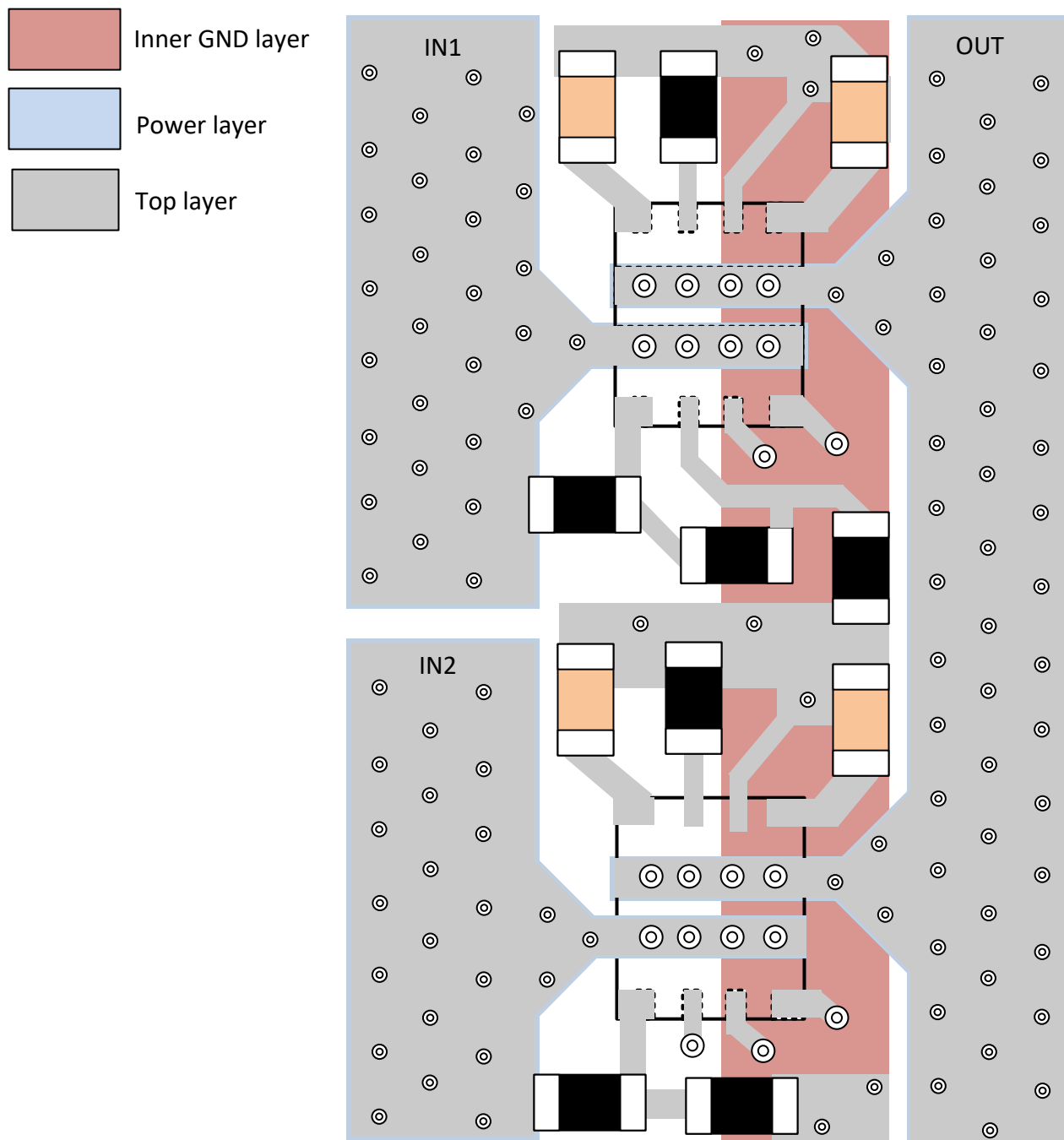
图 11-2. Layout Example - 2 × TPS259470x in PowerMUX Configuration
