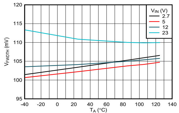
图 7-21. RCB - Forward Comparator Threshold vs Temperature
