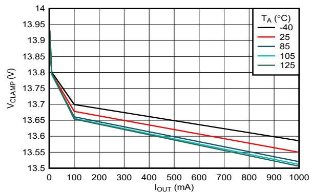
图 7-25. OVC Clamping Voltage (OVCSEL = 392 kΩ to GND) vs Load Current
