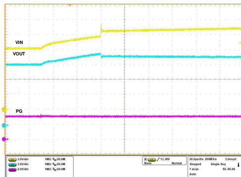
图 7-46. Overvoltage Clamp Response - TPS259472x
