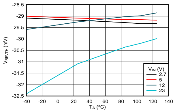
图 7-20. RCB - Reverse Comparator Threshold vs Temperature
