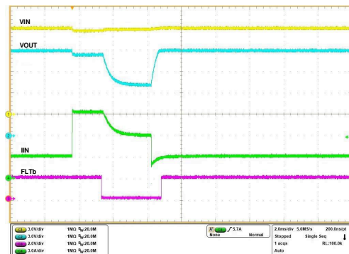
图 7-47. Overvoltage Clamp Response - TPS259472x
