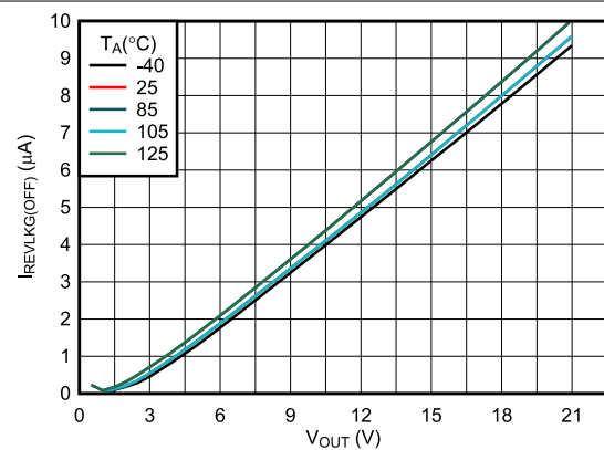
图 7-23. Reverse Leakage Current During OFF-State
