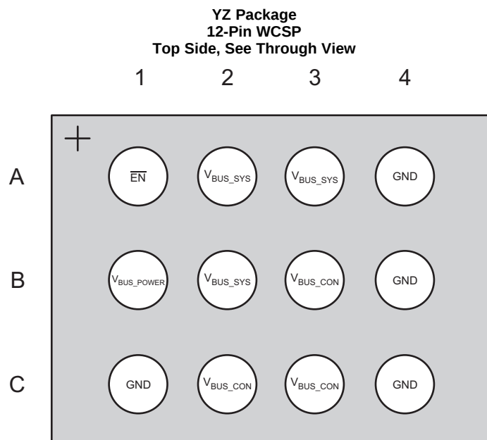
Pin Functions
