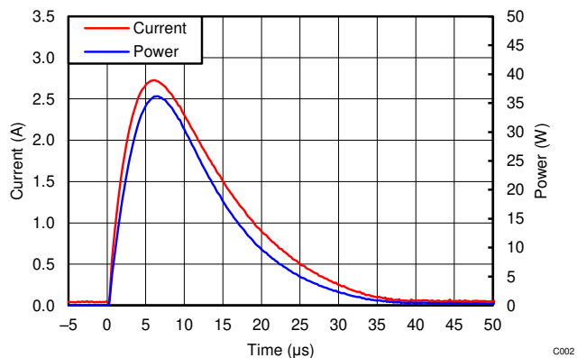
图 6-2. Surge Curve ( t_p = 8/20 \mu s ), Pin IO to GND
