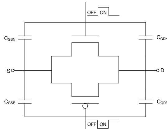
图 9-1. Transmission Gate Topology
