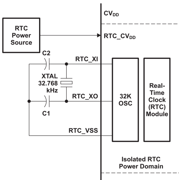
Figure 6-71. Clock Source
