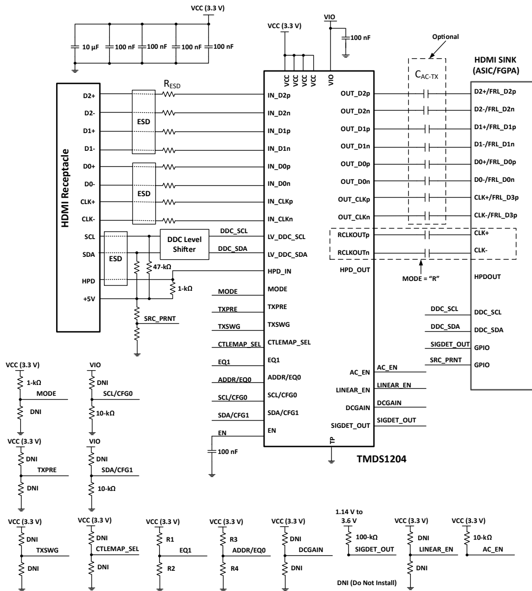
Figure 9-10. TMD51204 in Sink Application Schematics
