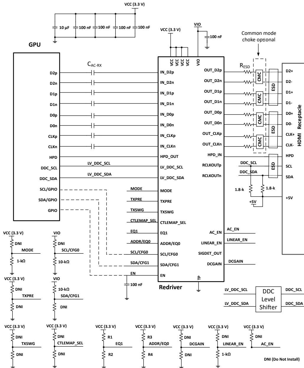
Figure 9-2. TMD51204 in Source Application Schematics
