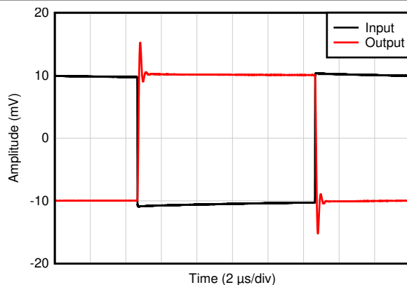
C_L = 20\text{pF} , G = -1 , 20\text{mV}_{pp} 阶跃响应
