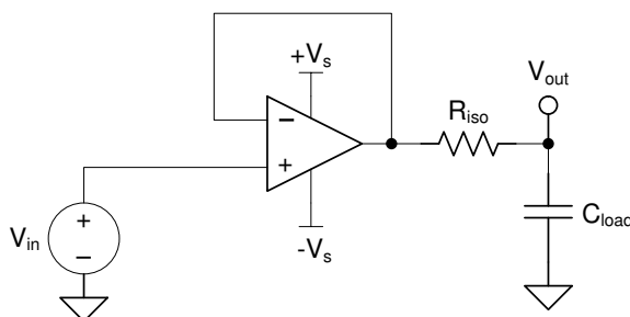
Figure 7-7. Extending Capacitive Load Drive With the OPA4991-EP
