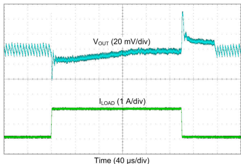
图 8-14. Buck Transient From PFM-to-PWM Mode
