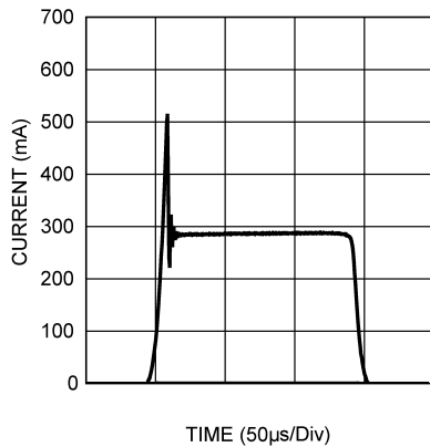
Figure 9. Short-Circuit Current
