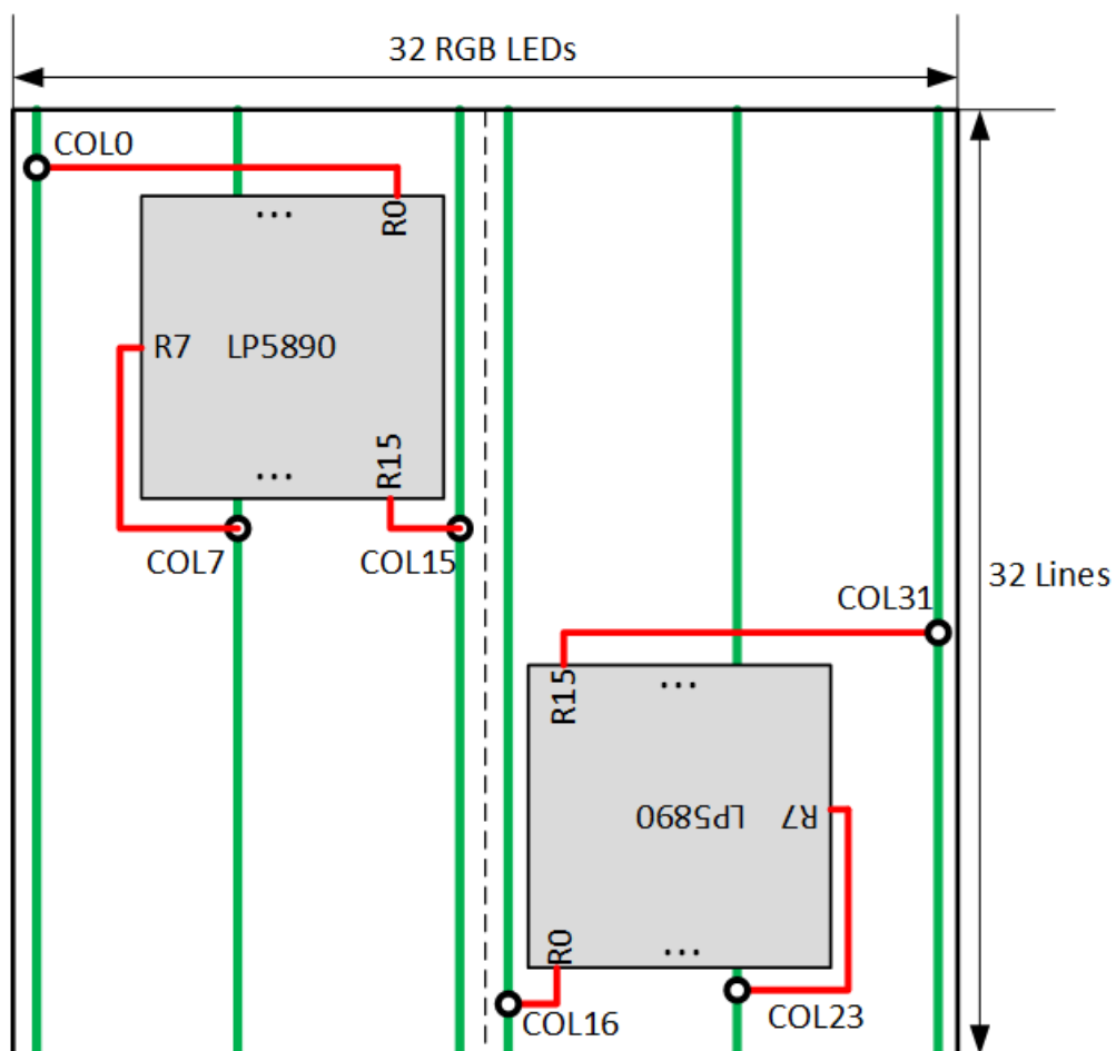
图 11-4. Channel Routing Suggestion with Channel Order Sequence
