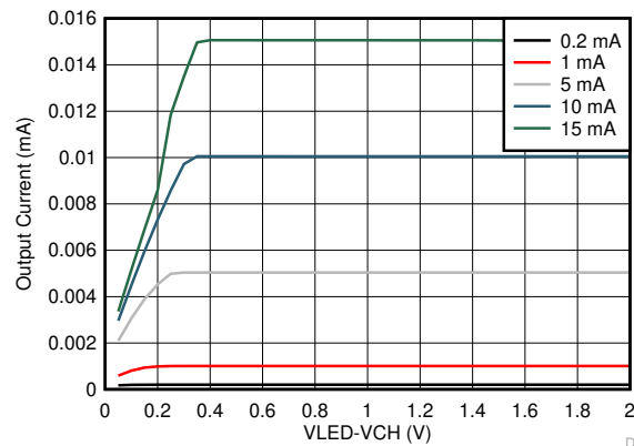
图 7-3. Channel Current vs (VLED-Vchannel) Voltage
