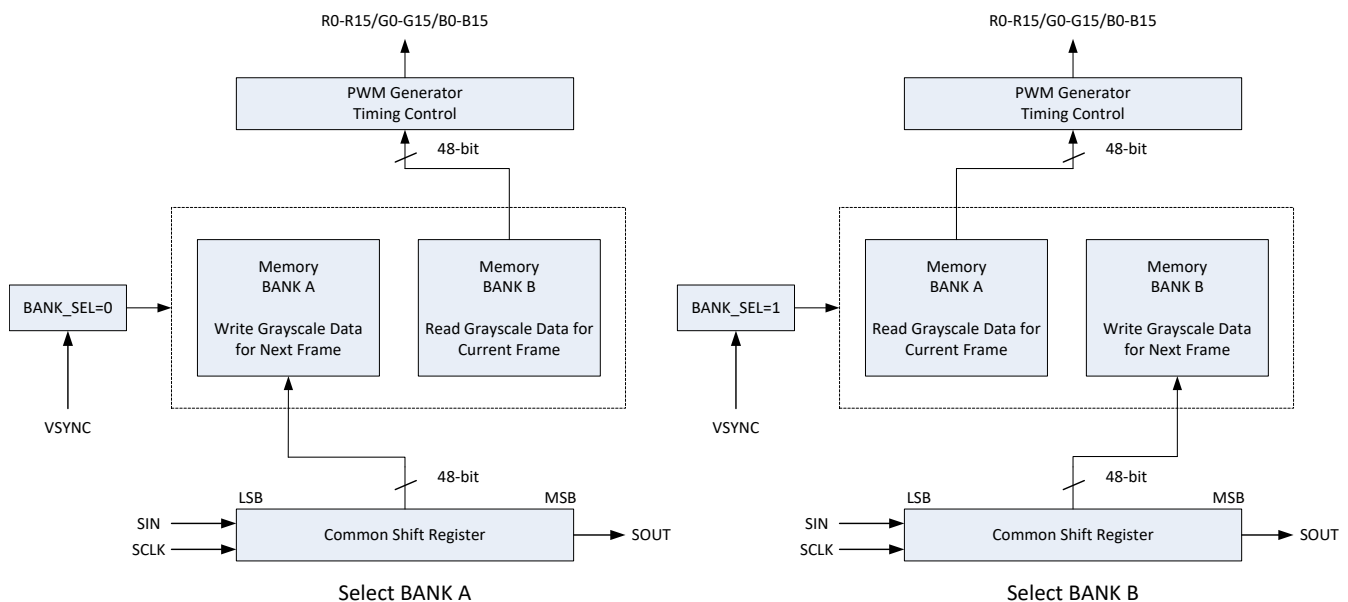
图 8-22. Bank Selection Exchange Operation
