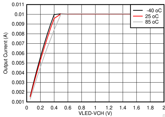
图 7-2. Channel Current vs (VLED-Vchannel) Voltage
