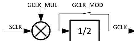
图 8-4. Frequency Multiplier Block Diagram
