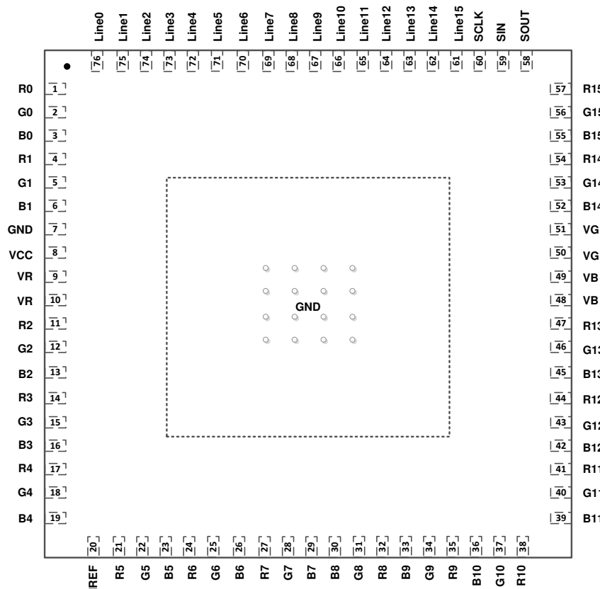
图 6-1. LP5890 RRF Package 76-Pin VQFN With Exposed Thermal Pad Top View
