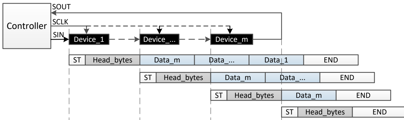
图 8-19. Data Write Command With Non-Broadcast
