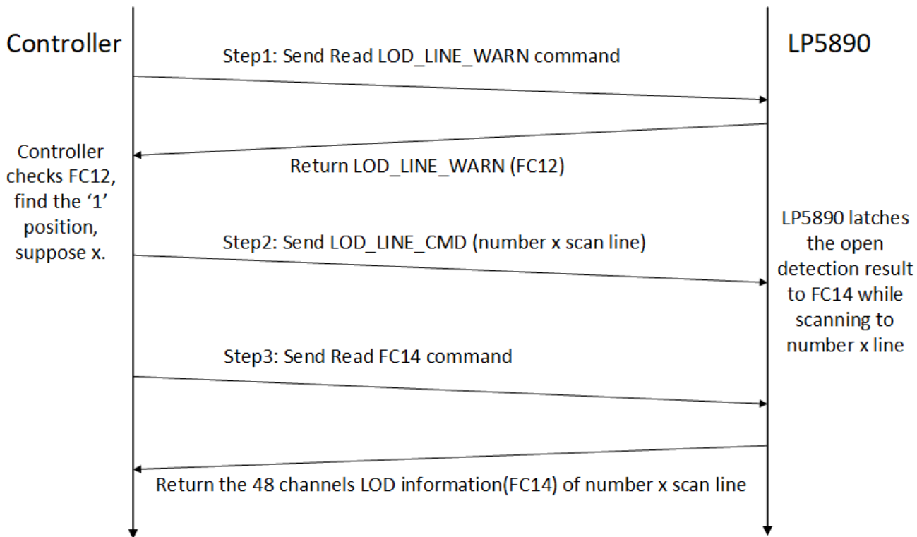
图 8-7. Steps to Read LED Open Information
