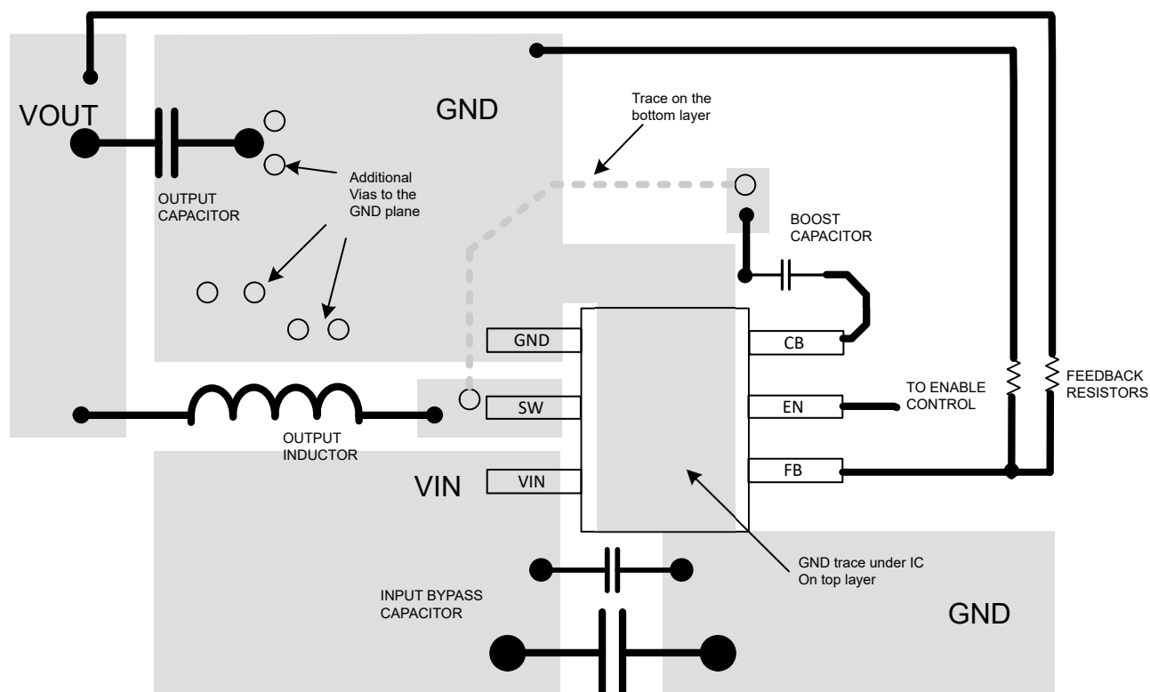
Figure 9-10. Layout
