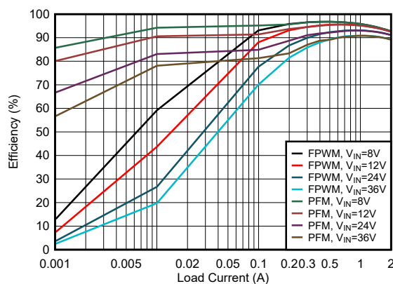
Efficiency vs Output Current, V_{OUT} = 5\text{ V} , 500 kHz
