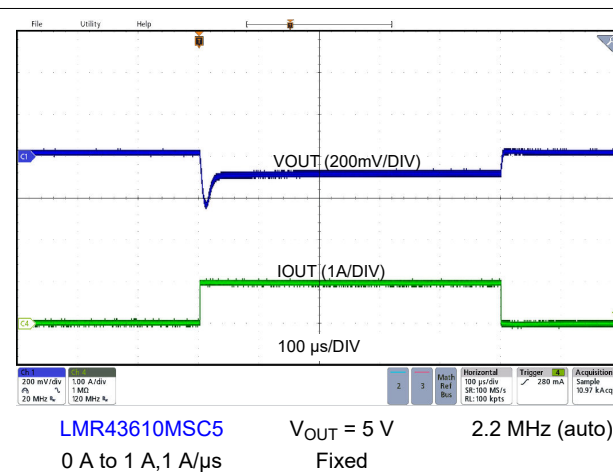
Figure 9-20. Load Transient
