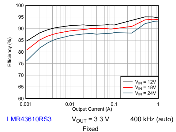
Figure 9-8. Efficiency
