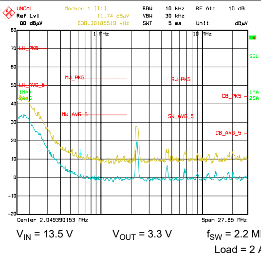
Figure 9-25. Typical CISPR 25 Conducted EMI 150 kHz–30 MHz Yellow: Peak Detect, Blue = Average Detect
