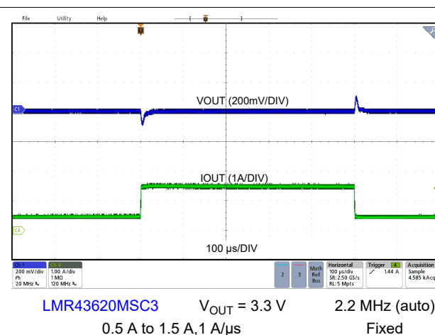
Figure 9-16. Load Transient
