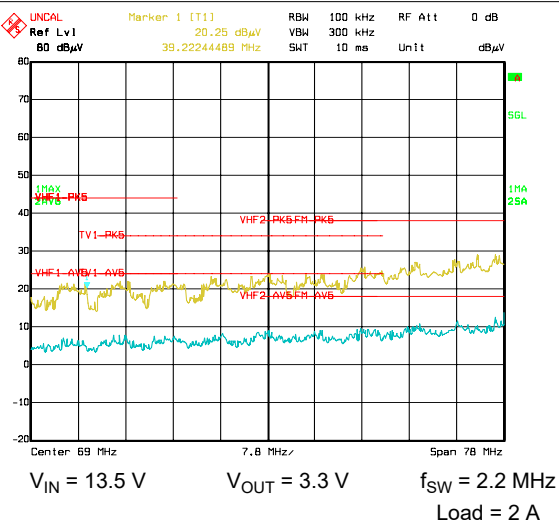
Figure 9-26. Typical CISPR 25 Conducted EMI 30 MHz–108 MHz Yellow: Peak Detect, Blue = Average Detect
