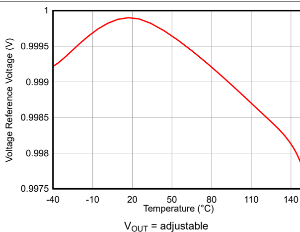
Figure 7-4. Feedback Voltage Accuracy Versus Temperature
