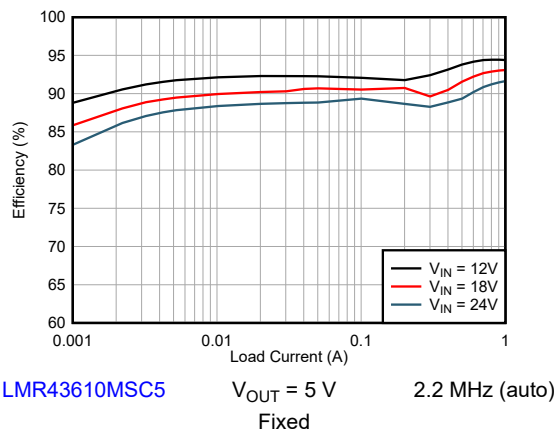
Figure 9-5. Efficiency
