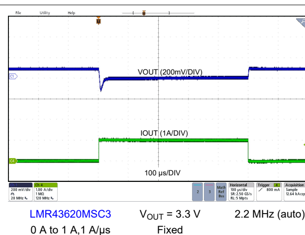
Figure 9-18. Load Transient
