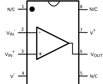
D Package 8-Pin Single SOIC Top View
