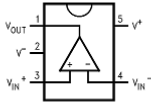
DBV Package 5-Pin SOT-23 Single Top View
