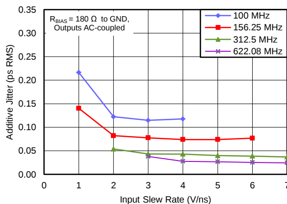
Figure 4. Additive Jitter vs Input Slew Rate
