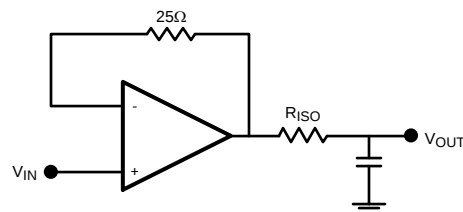
Figure 41. Isolation Resistor Placement
