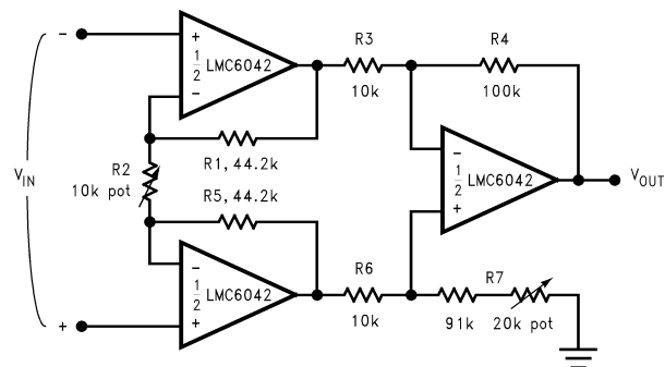
Figure 41. Instrumentation Amplifier
