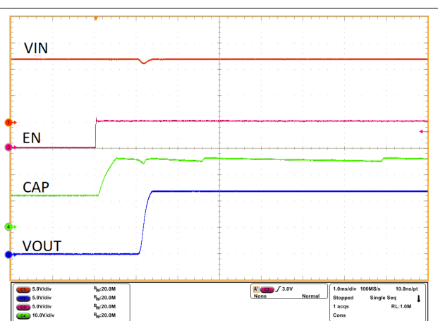
Figure 9-6. Startup with EN Going Low to High
