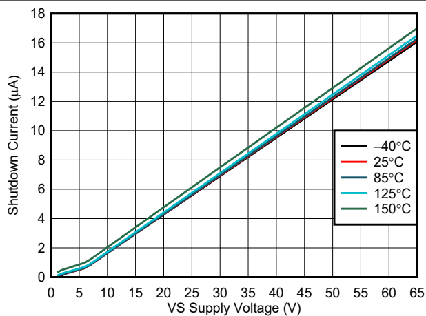
Figure 6-2. Shutdown Current vs Supply Voltage
