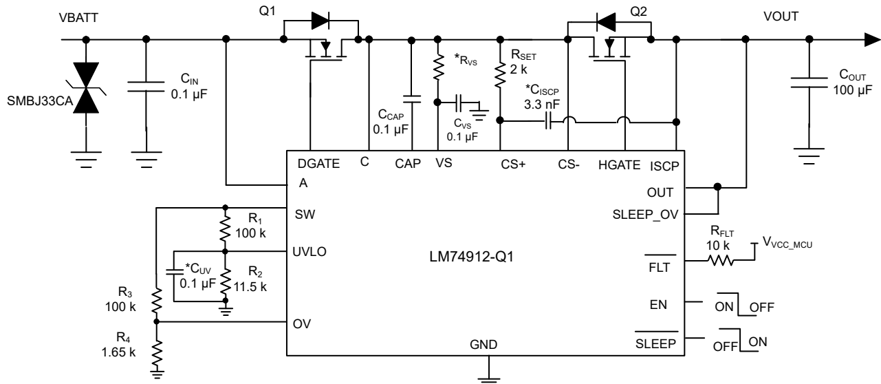
Figure 9-1. Typical Application Circuit – 12-V Reverse Battery Protection and Overvoltage Protection
