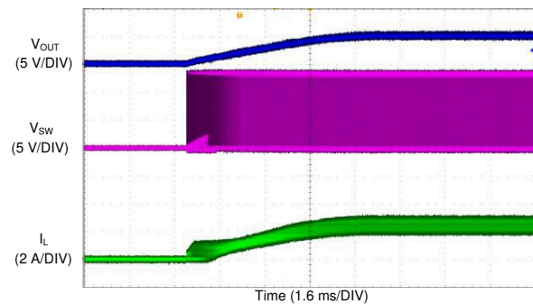
图 9-20. Short Circuit Recovery
