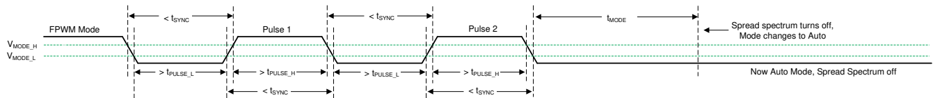
图 9-8. Spread Spectrum Disabled in Transition from FPWM Mode to Auto Mode
