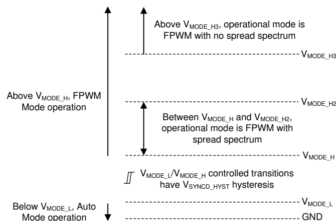
图 9-2. Level-Dependent Mode Selection Settings
