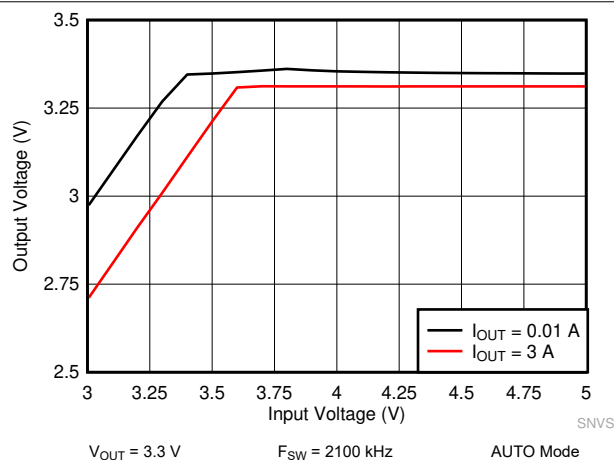
图 10-13. LM62440-Q1 Dropout Curve
