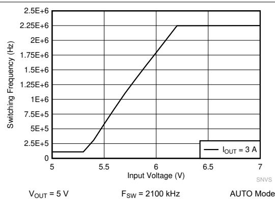
图 10-16. LM62440-Q1 Frequency Dropout Curve
