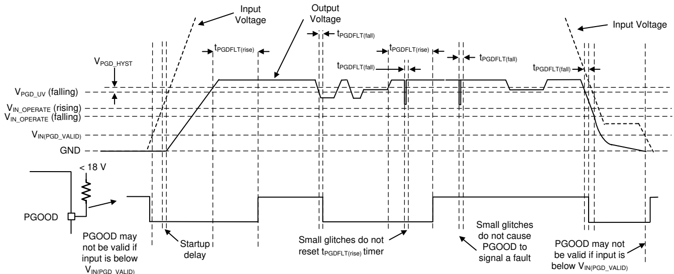
图 9-13. PGOOD Timing Diagram (Excludes OV Events)
