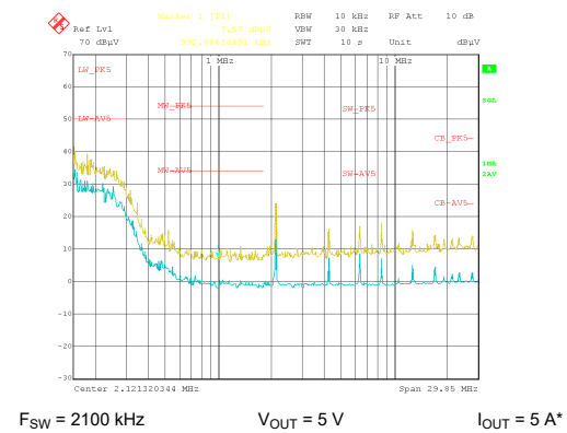
图 10-32. Radiated EMI Log Horizontal versus CISPR25 Limits
