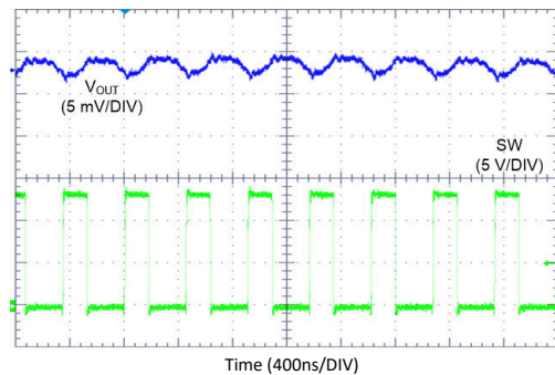
图 10-18. LM62440-Q1 Switching Waveform and V_{OUT} Ripple
