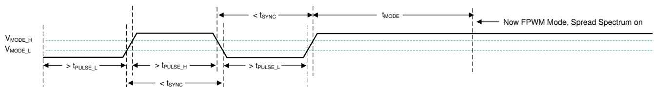
图 9-11. Transition from SYNC Mode to FPWM Mode
