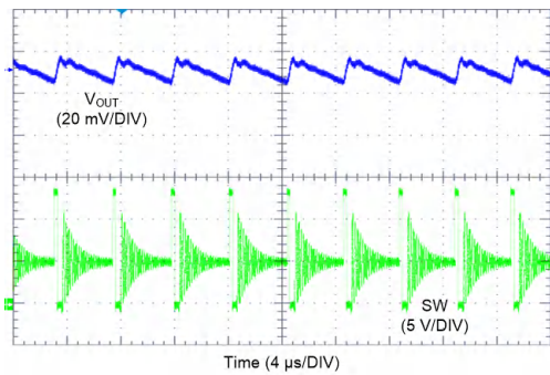
图 10-17. LM62440-Q1 Switching Waveform and V_{OUT} Ripple
