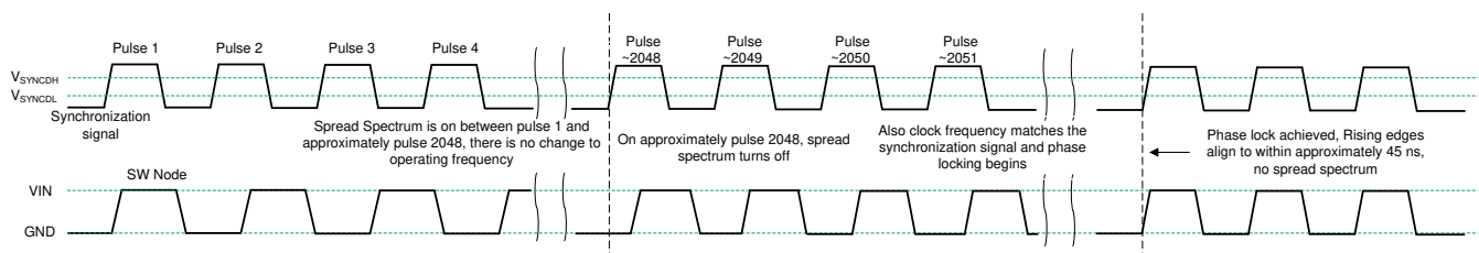
图 9-12. Synchronization Process
