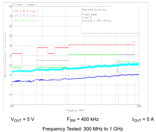
图 10-32. Radiated EMI Log Horizontal versus CISPR25 Limits
