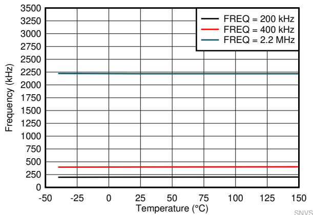
图 8-5. Switching Frequency Set by SYNC
