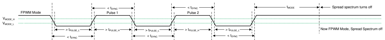
图 9-6. Spread Spectrum Disabled in FPWM Mode
