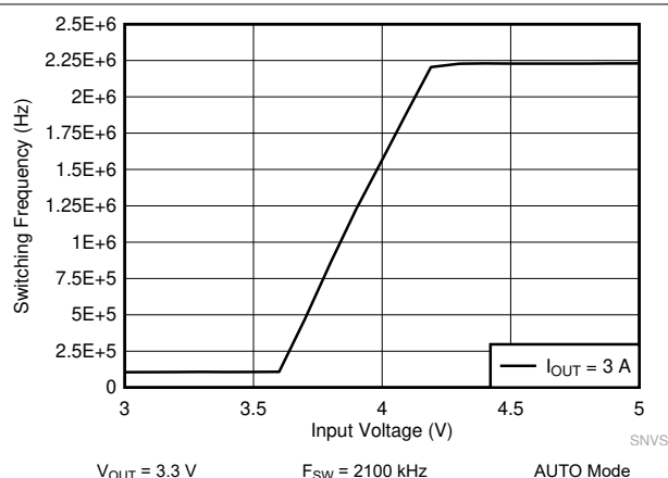
图 10-15. LM62440-Q1 Frequency Dropout Curve
