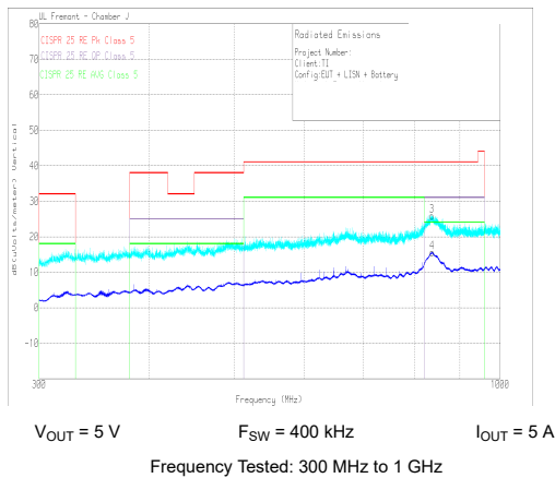
图 10-31. Radiated EMI Log Vertical versus CISPR25 Limits
