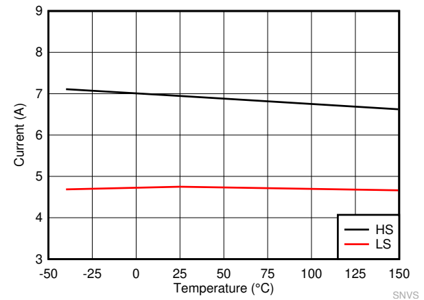
图 8-4. LM62440-Q1 High-side and Low-side Current Limits
