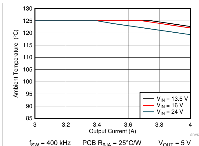
图 10-2. Maximum Ambient Temperature versus Output Current
