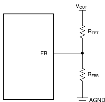
图 9-17. Setting Output Voltage of Adjustable Versions
