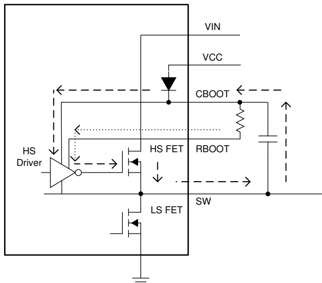
图 9-14. Simplified Circuit Showing How RBOOT Functions
