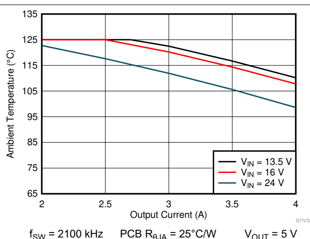
图 10-3. Maximum Ambient Temperature versus Output Current
