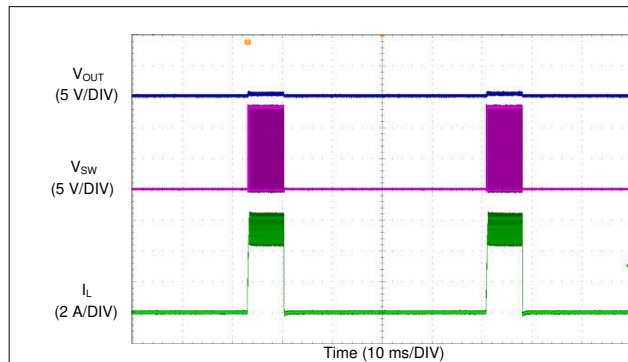
图 9-19. Inductor Current Bursts During Hiccup
