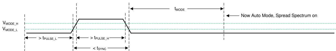
图 9-10. Transition from SYNC Mode to Auto Mode
