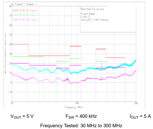
图 10-30. Radiated EMI Bicon Horizontal versus CISPR25 Limits
