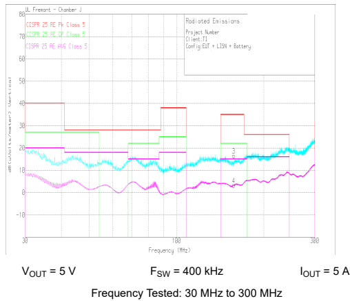
图 10-29. Radiated EMI Bicon Vertical versus CISPR25 Limits
