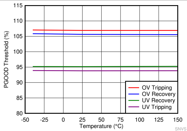
图 8-8. PGOOD Thresholds
