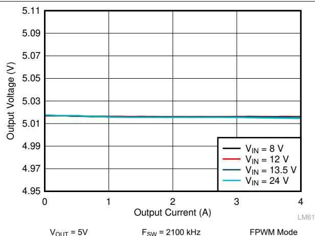
图 10-12. LM62440-Q1 Load and Line Regulation
