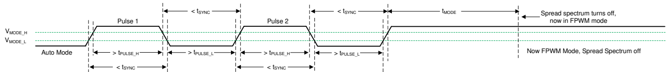
图 9-9. Spread Spectrum Disabled in Transition from Auto Mode to FPWM Mode
