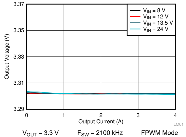
图 10-12. LM61440-Q1 Load and Line Regulation
