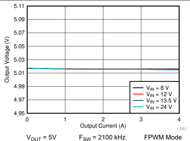
图 10-16. LM61440-Q1 Load and Line Regulation
