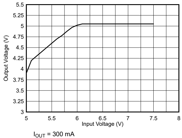
Figure 9-32. Drop-Out Response
