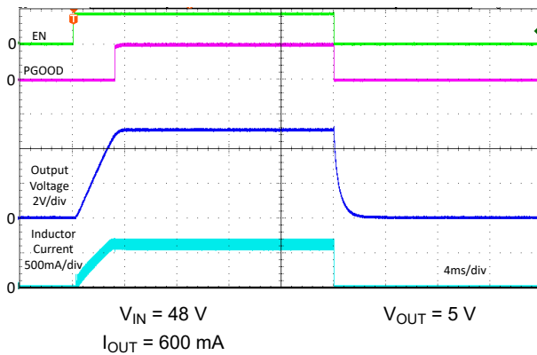
Figure 9-29. Typical Start-up Waveforms
