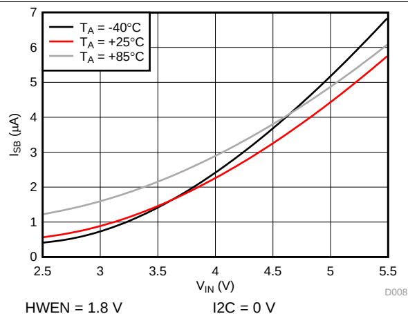
Figure 17. Shutdown Current vs Input Voltage
