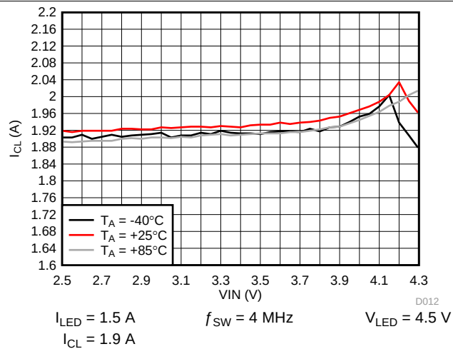
Figure 22. Inductor Current Limit vs Input Voltage
