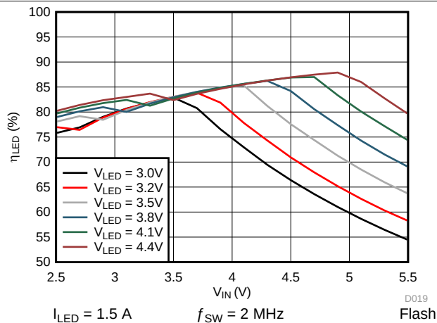
Figure 37. 2-MHz LED Efficiency vs Input Voltage
