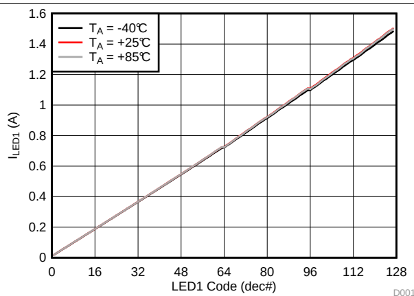
Figure 2. LED1 Flash Current vs Brightness Code
