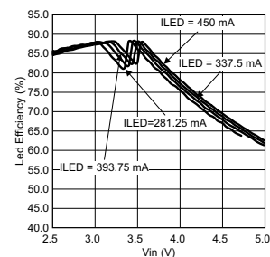
LED 效率与 V_{IN} 双 LED
