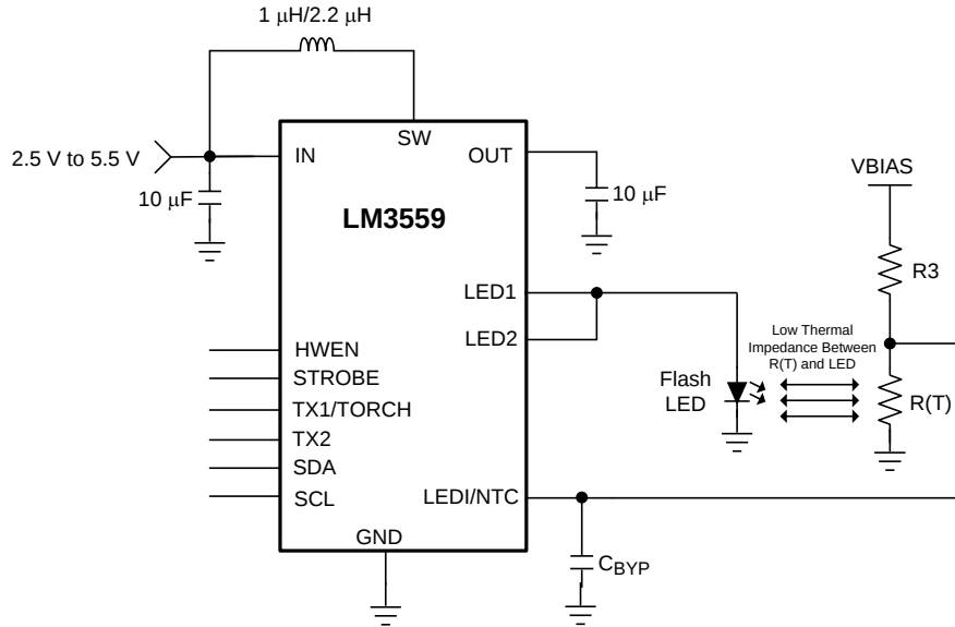
Figure 48. LM3559 Typical Application Circuit With Thermistor
