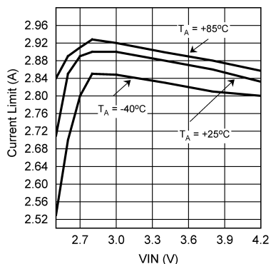
Figure 1. Closed Loop Current Limit vs V_{IN} Flash Duration
