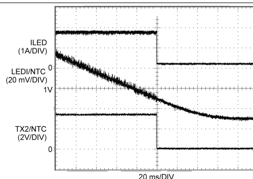
Figure 20. NTC-Mode Operation
