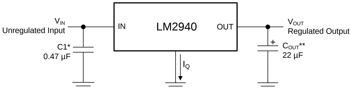
Simplified Schematic
