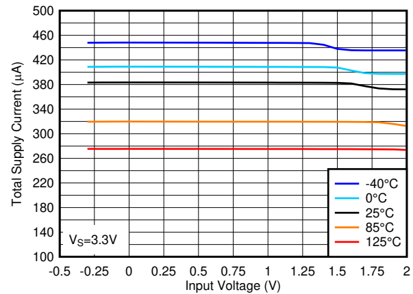
图 3-9. Total Supply Current vs. Input Voltage at 3.3V
