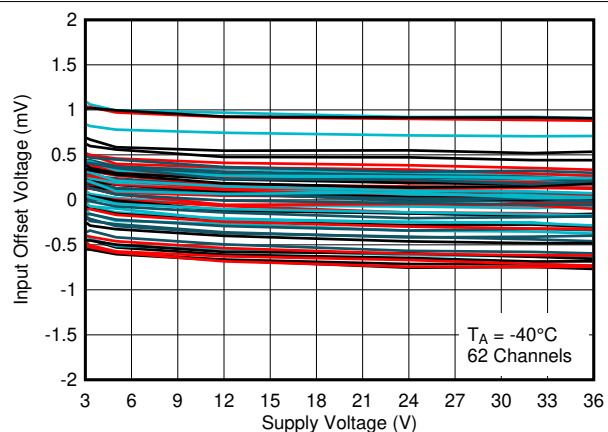
图 3-17. Input Offset Voltage vs. Supply Voltage at -40^\circ\text{C}
