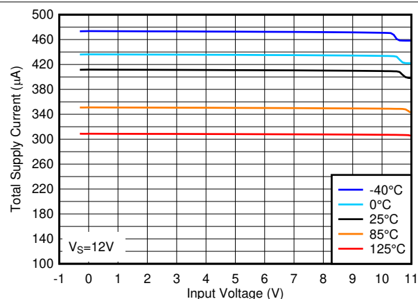
图 3-11. Total Supply Current vs. Input Voltage at 12V
