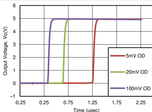
图 5-2. Response Time for Various Overdrives (Positive Transition)
