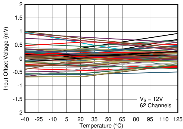
图 3-15. Input Offset Voltage vs. Temperature at 12V
