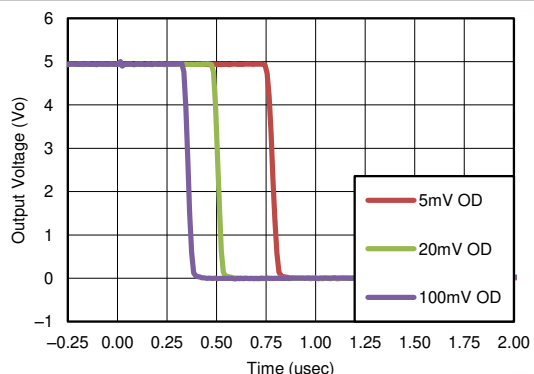
图 5-3. Response Time for Various Overdrives (Negative Transition)
