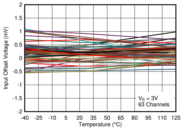
图 3-13. Input Offset Voltage vs. Temperature at 3V
