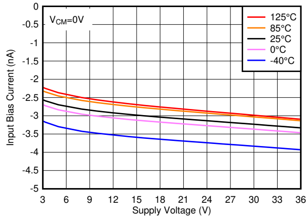
图 3-21. Input Bias Current vs. Supply Voltage
