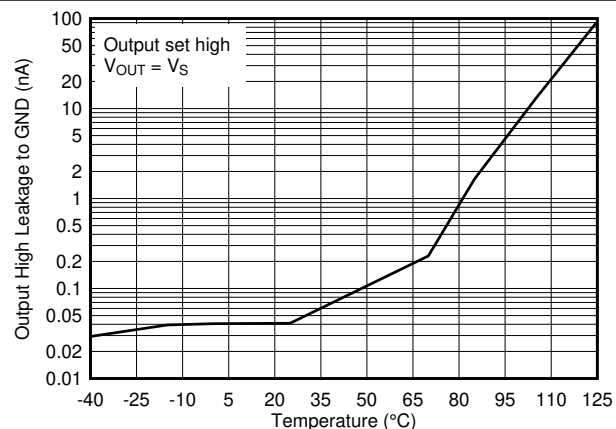
图 3-29. Output High Leakage Current vs. Temperature at 5V
