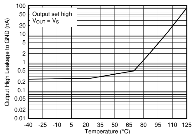
图 3-30. Output High Leakage Current vs. Temperature at 36V
