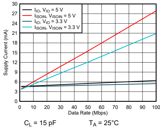
图 7-11. ISOW7740 Channel Supply Currents vs Data Rate For C_L = 15\text{ pF}
