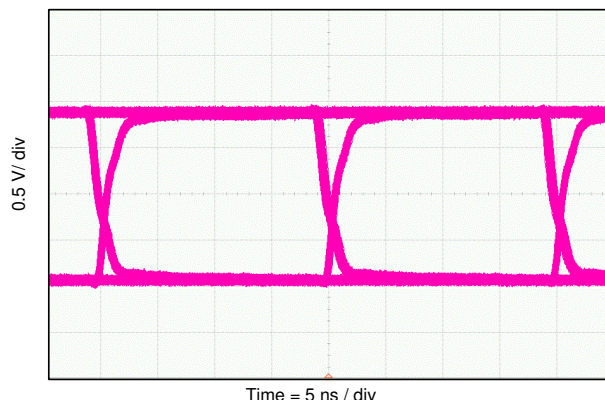
图 10-6. Eye Diagram at 50 Mbps PRBS 2^{16} - 1 , 1.8 V and 25°C
