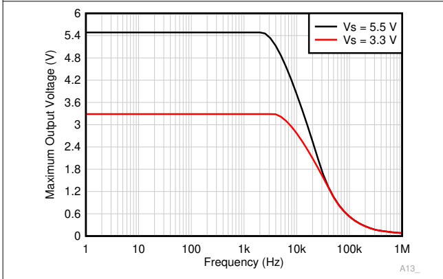
Figure 7-39. Maximum Output Voltage vs Frequency
