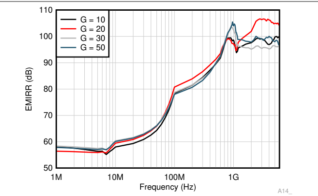
Figure 7-42. Electromagnetic Interference Rejection Ratio Referred to Noninverting Input (EMIRR+) vs Frequency
