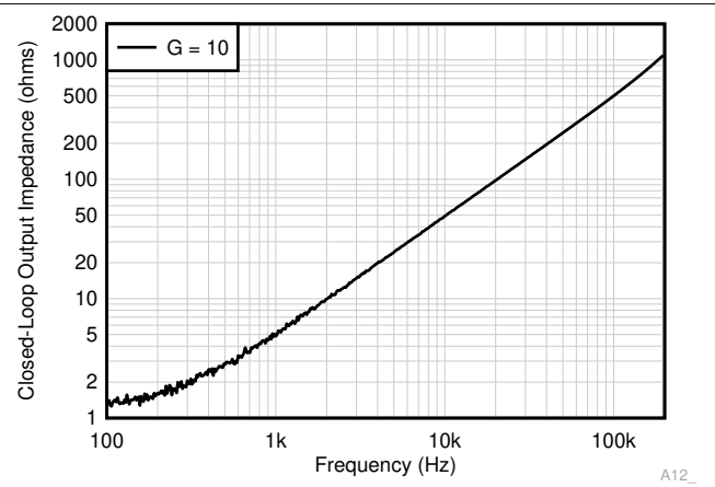
Figure 7-38. Closed-Loop Output Impedance vs Frequency
