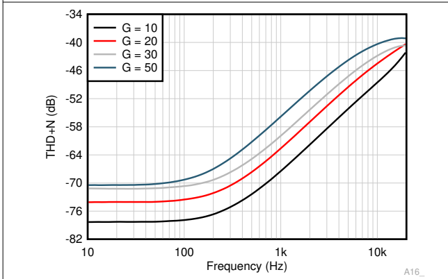
Figure 7-41. THD + N Frequency
