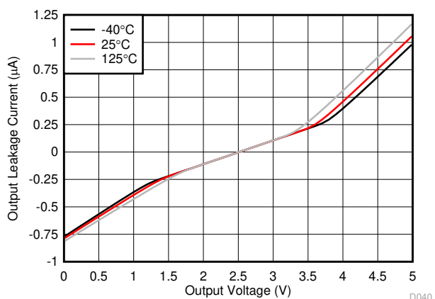
V_S = 5.0\text{V} , V_{\text{ENABLE}} = 0\text{V} , V_{\text{REF}} = 2.5\text{V}
