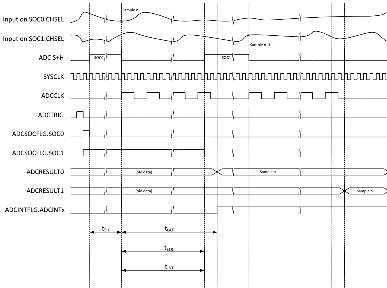
图 7-33. ADC Timings for 12-Bit Mode
