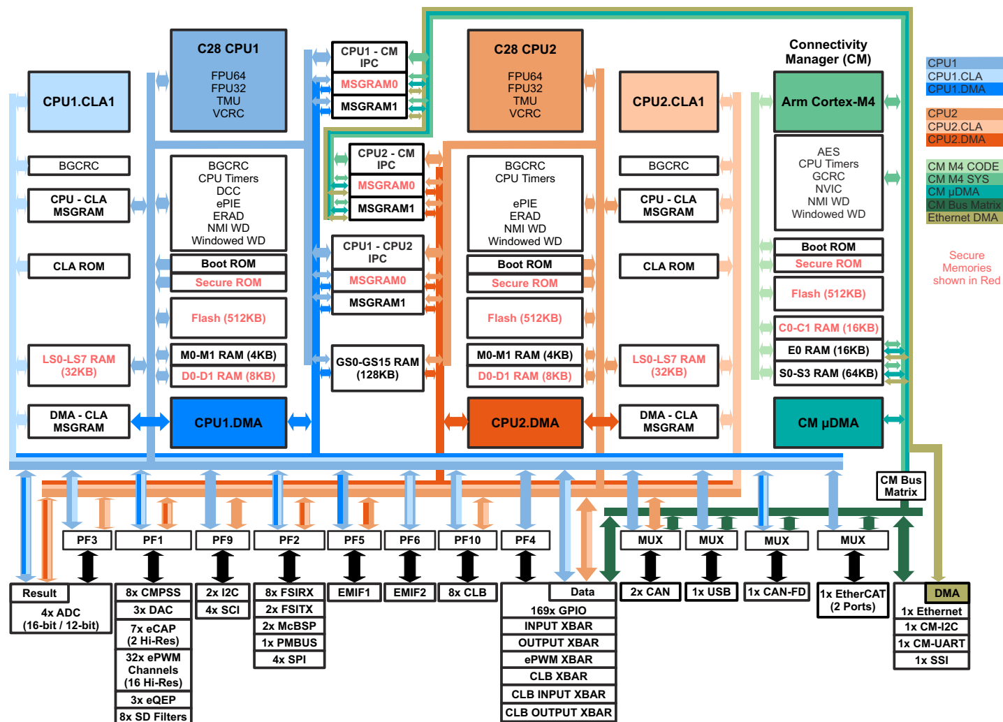
图 8-1. Functional Block Diagram
