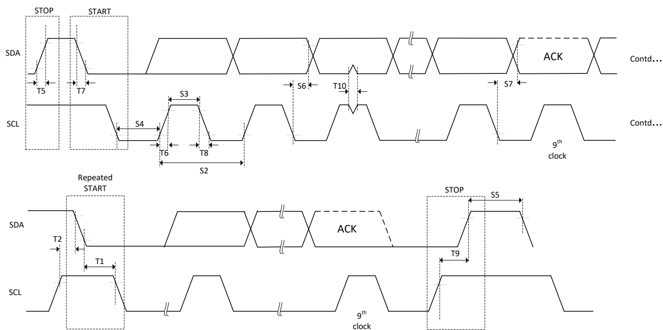
图 7-67. I2C Timing Diagram
