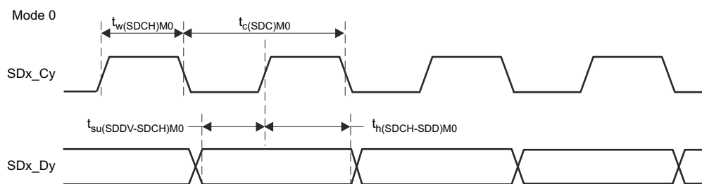
图 7-57. SDFM Timing Diagram - Mode 0
