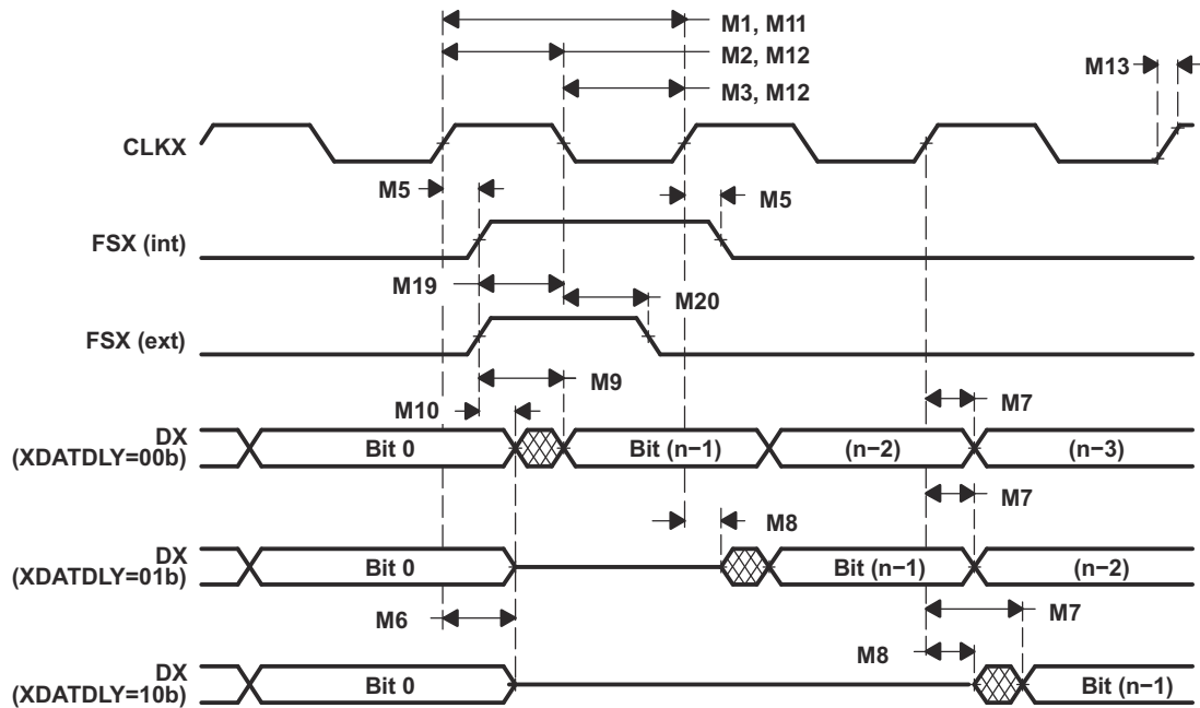
图 7-70. McBSP Transmit Timing
