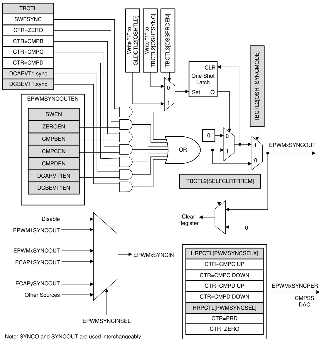
图 7-52. Synchronization Chain Architecture
