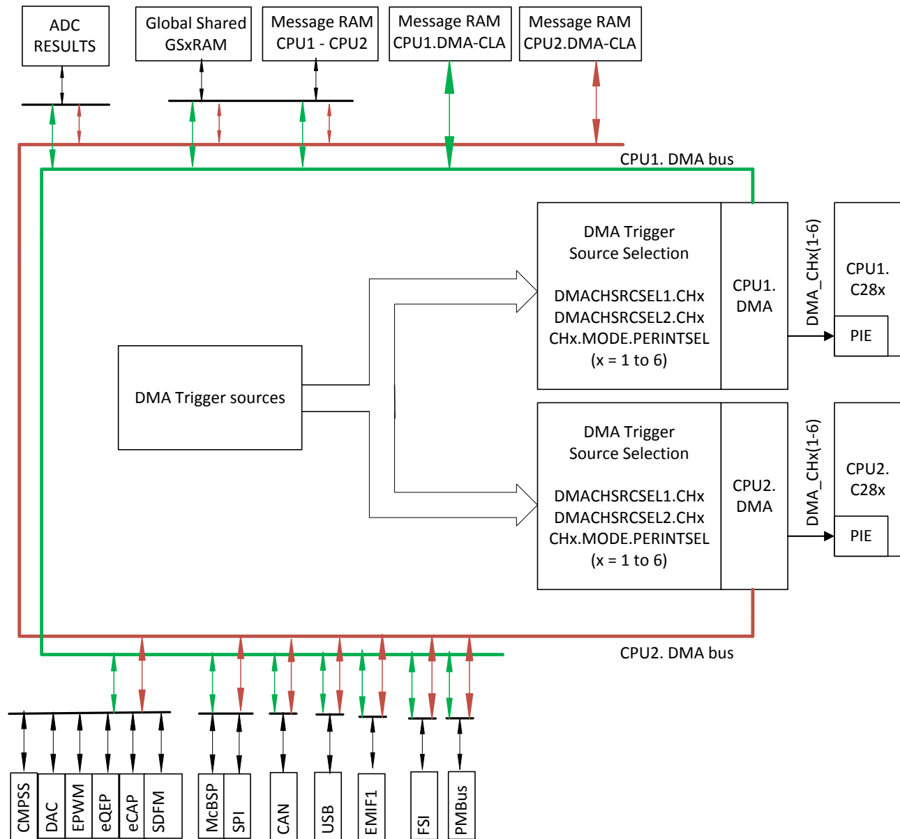
图 8-5. DMA Block Diagram
