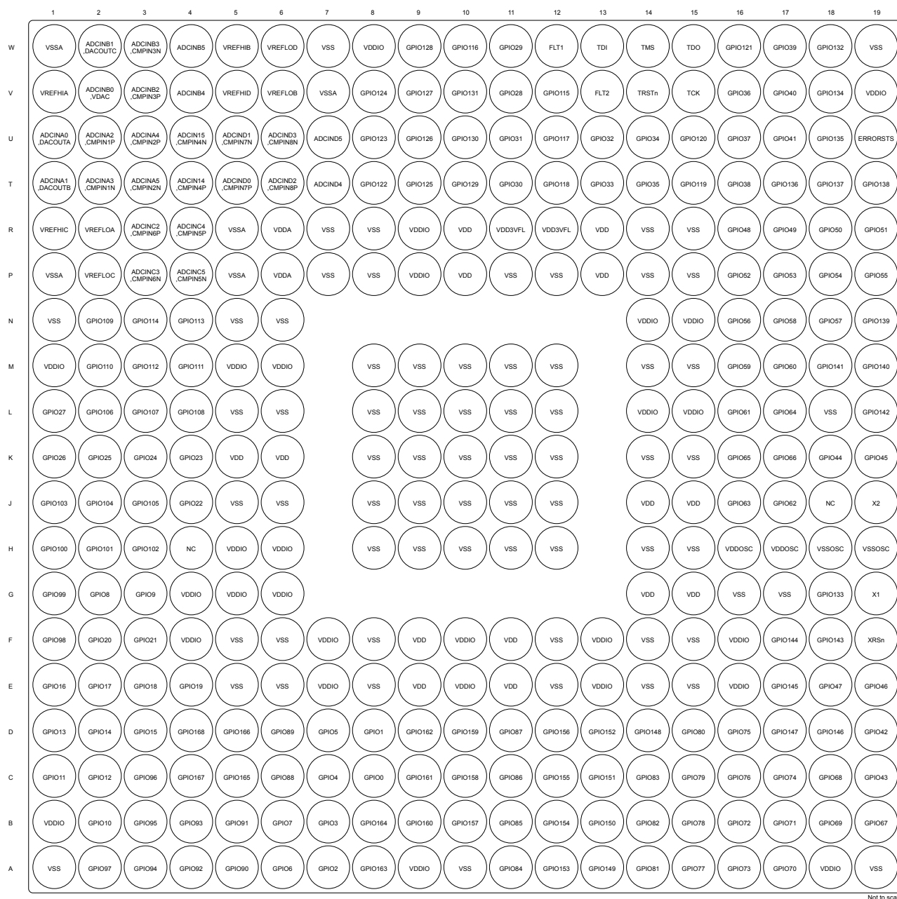
图 6-1. 337-Ball ZWT New Fine Pitch Ball Grid Array (Bottom View)
