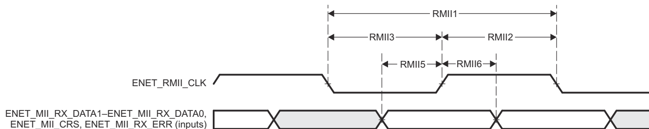
图 7-95. Receive Interface Timing (RMII Operation)
