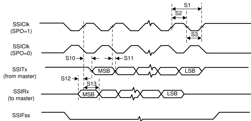
图 7-101. Master Mode SSI Timing for SPI Frame Format (FRF = 00), with SPH = 1
