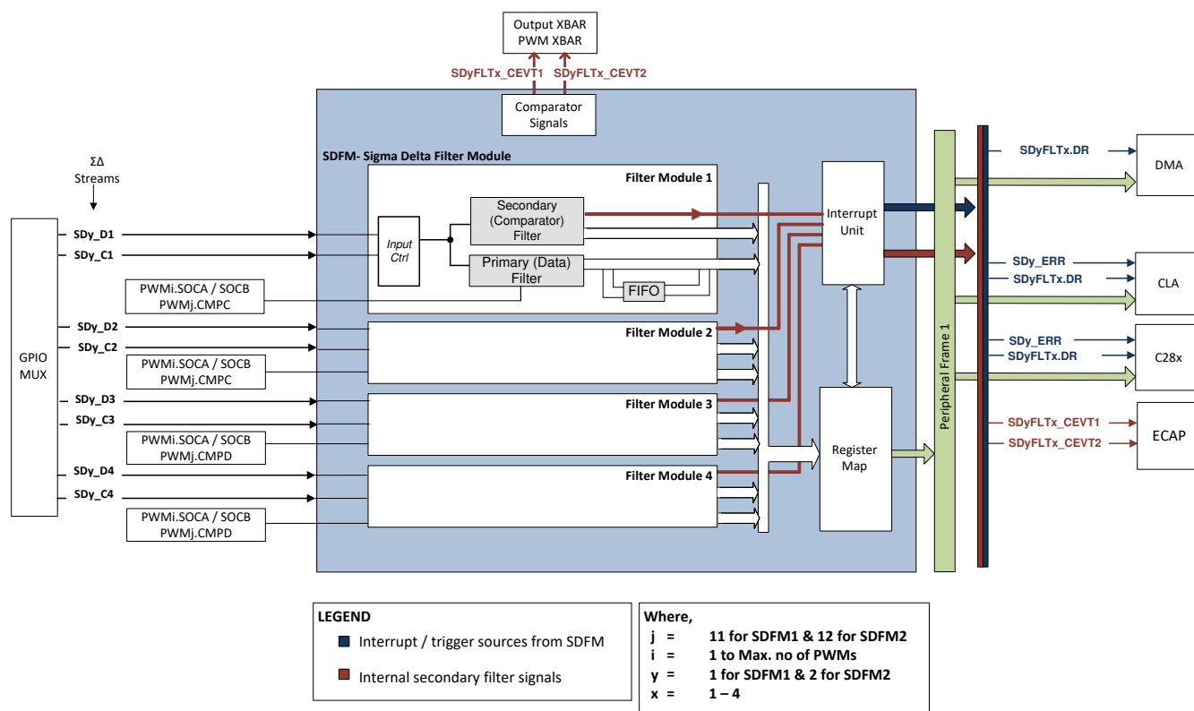
图 7-56. SDFM Block Diagram
