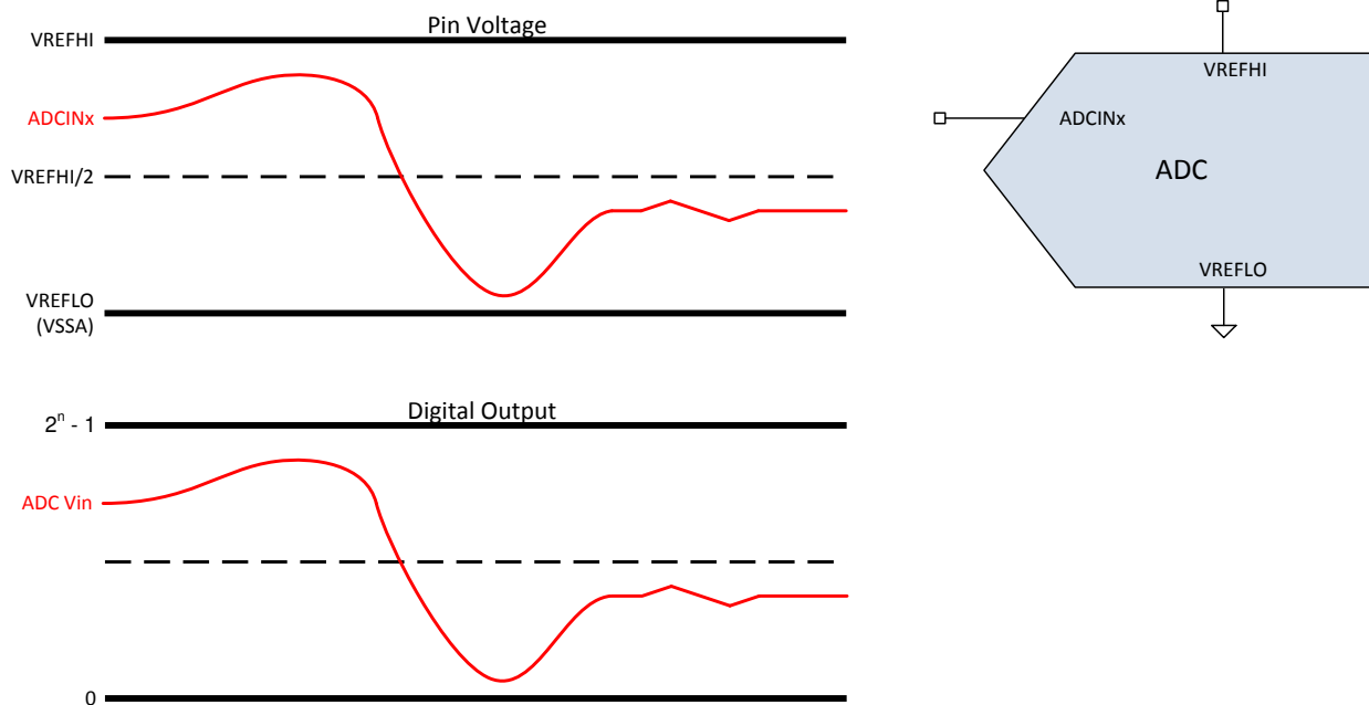
图 7-30. Single-ended Signaling Mode
