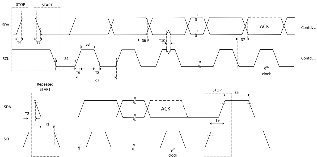
图 7-98. CM-I2C Timing Diagram
