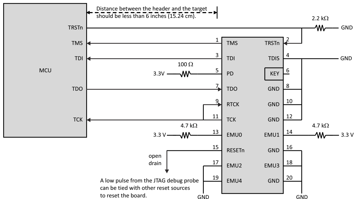
图 7-11. Connecting to the 20-Pin JTAG Header
