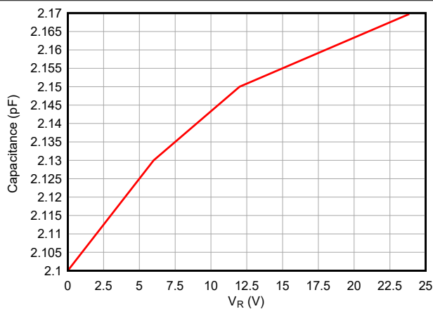
Figure 6-5. Capacitance vs. Bias Voltage
