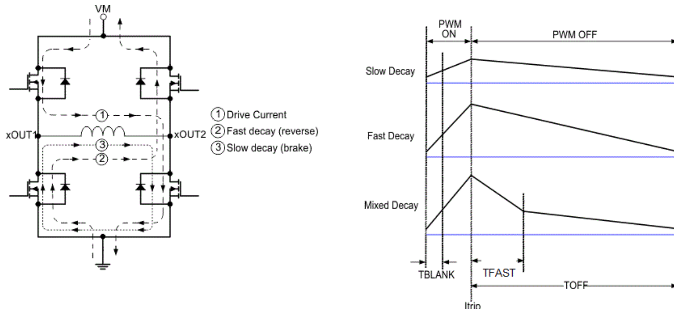
Figure 7-5. Decay Modes
