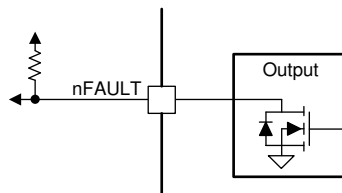
Figure 7-14. nFAULT Pin
