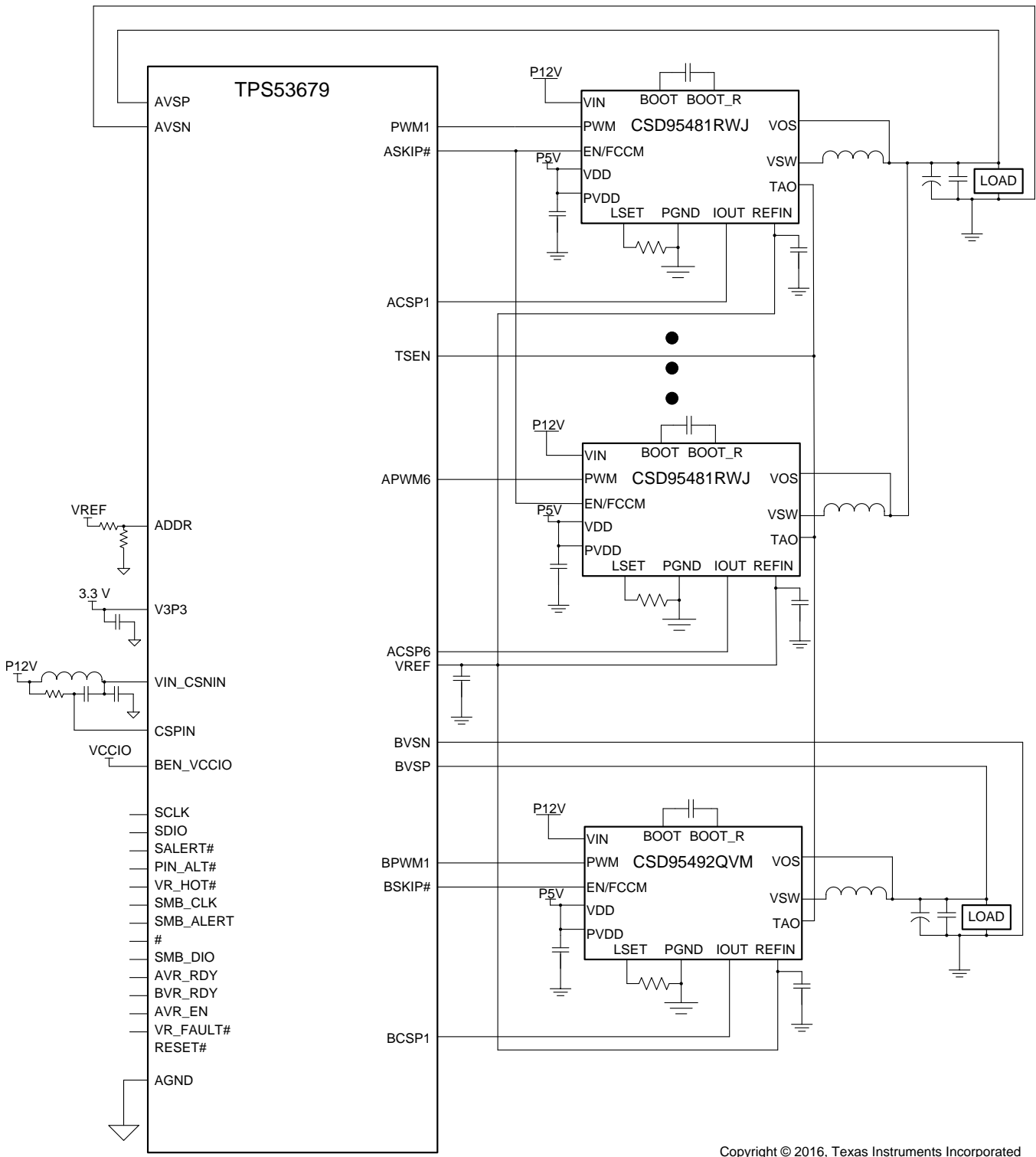
Figure 1. Application Schematic
