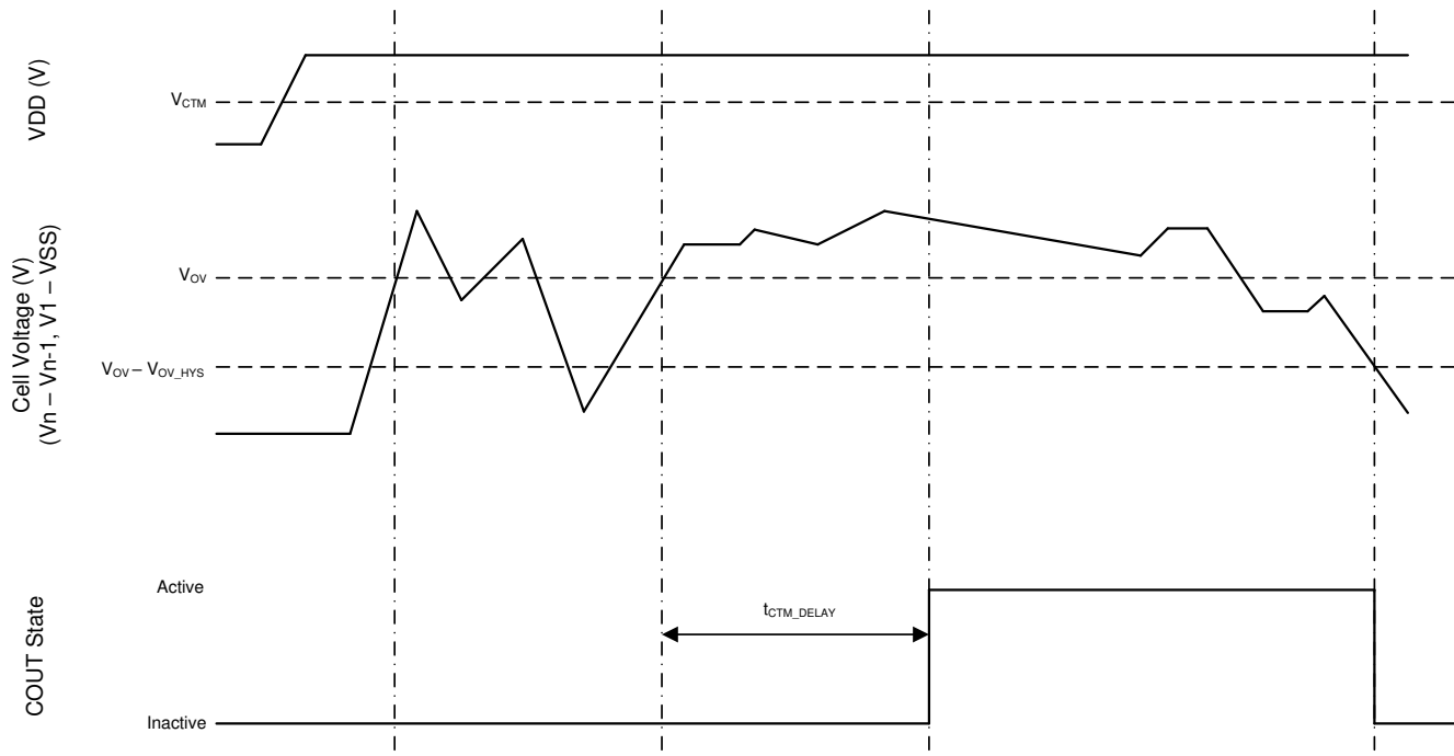
图 9-3. Timing for Customer Test Mode
