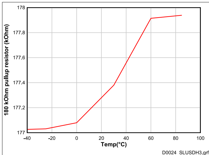
图 7-22. Thermistor Pullup Resistance vs. Temperature (180-kΩ setting)
