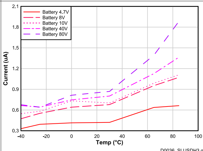
图 7-29. BAT Current in SHUTDOWN Mode vs. Temperature
