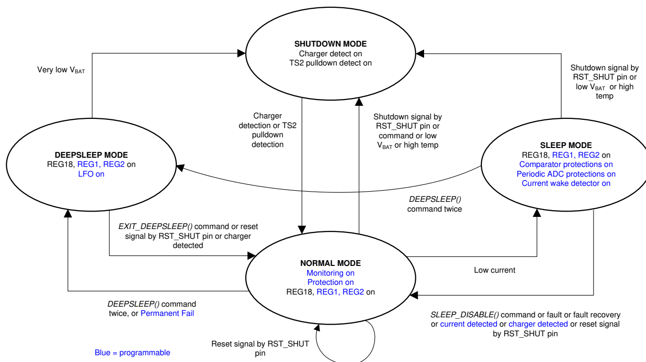
图 13-1. Device Functional Modes
