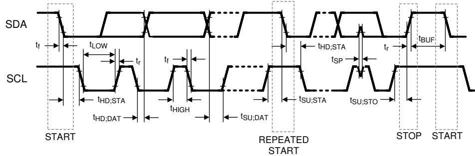
图 7-1. I²C Communications Interface Timing
