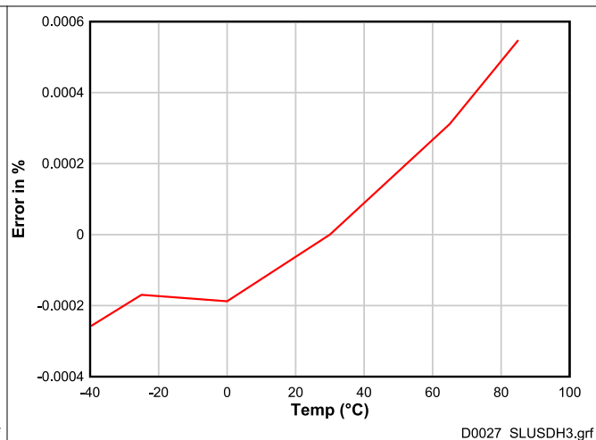
图 7-23. Coulomb Counter Gain Error vs. Temperature
