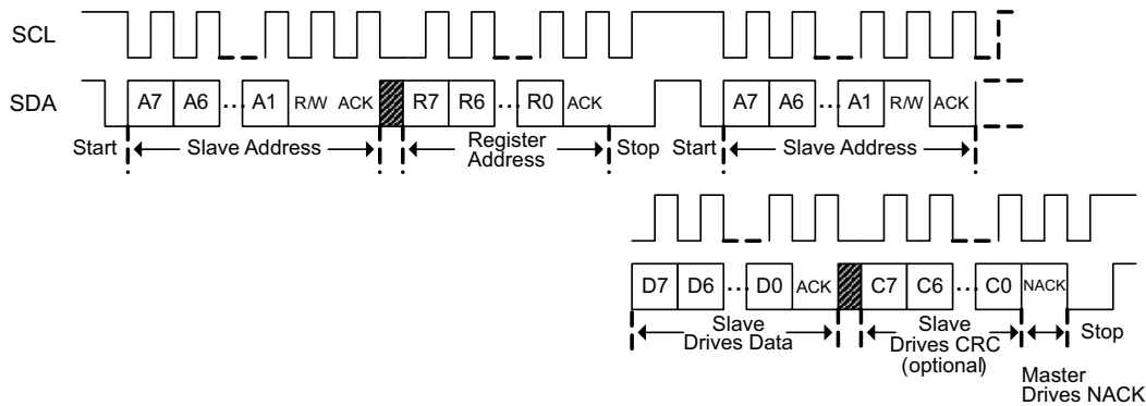
图 14-3. I²C Read Without Repeated Start
