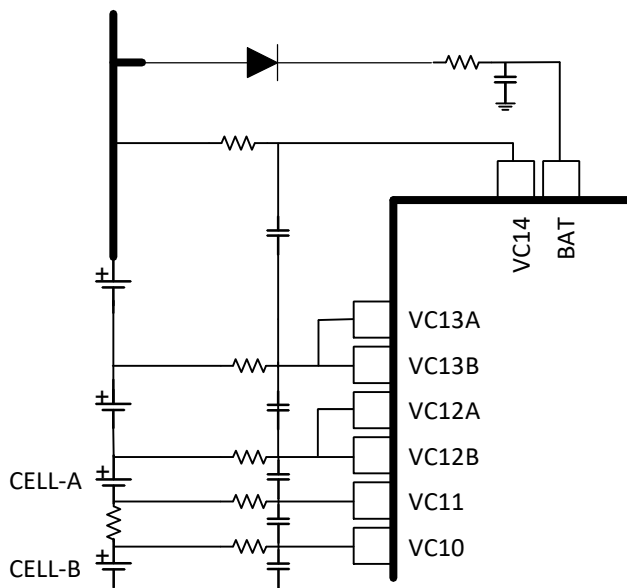
图 10-1. Using Cell Input Pins for Interconnect Measurement
