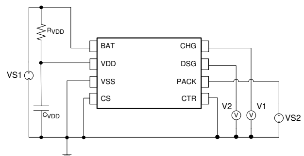
Figure 9-2. Test Circuit 2
