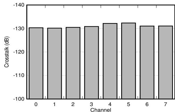
Figure 6-21. Crosstalk vs Channel
