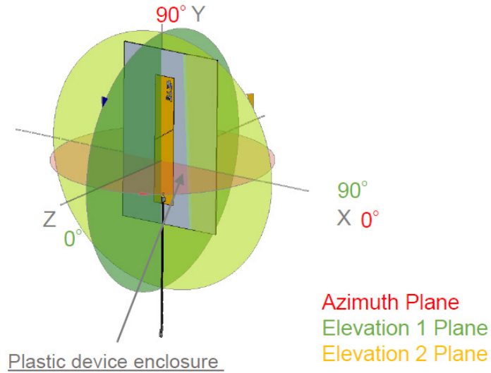
Test setup
