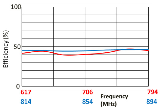
Efficiency
