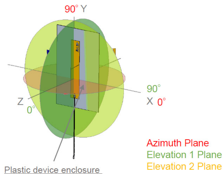
Test setup
