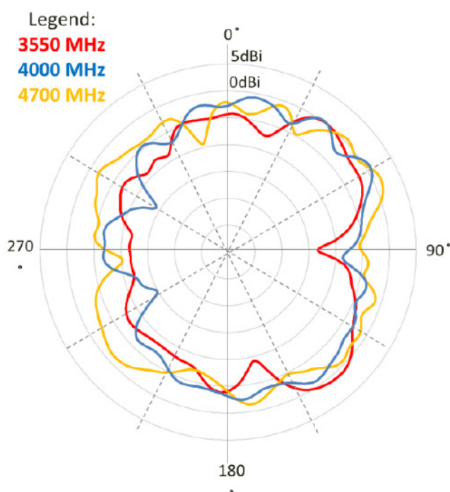
Elevation 2(YZ)
