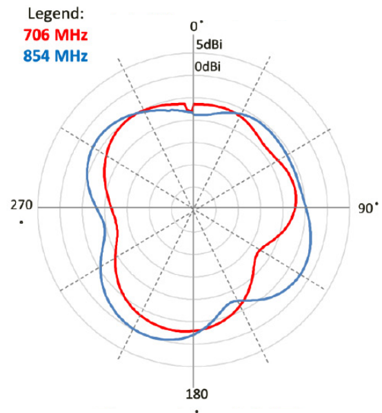
Azimuth(XY)
