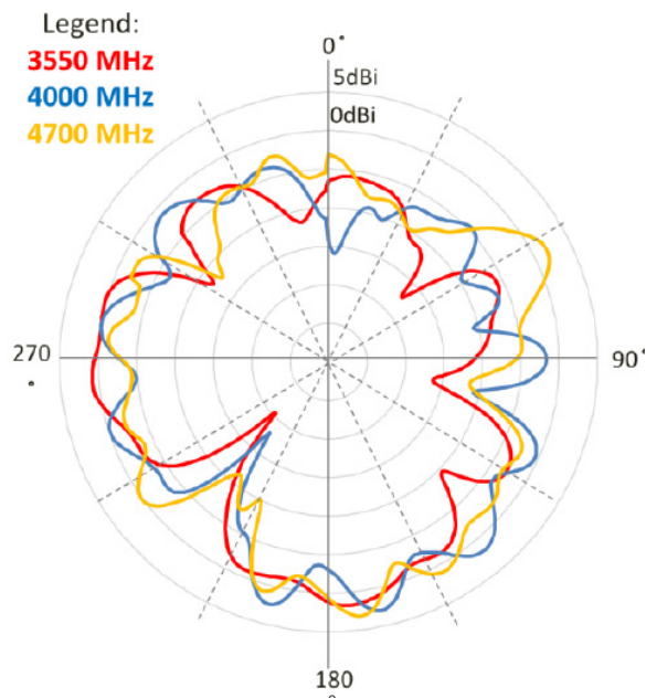
Azimuth(XY)
