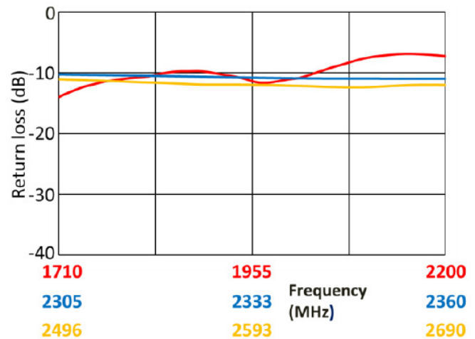
Return Loss
