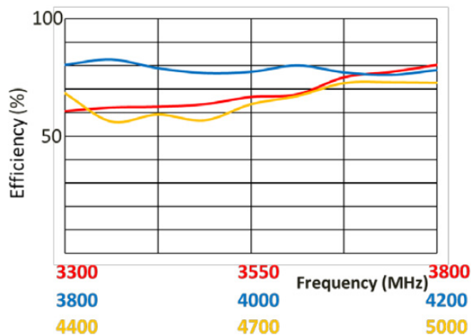
Efficiency
