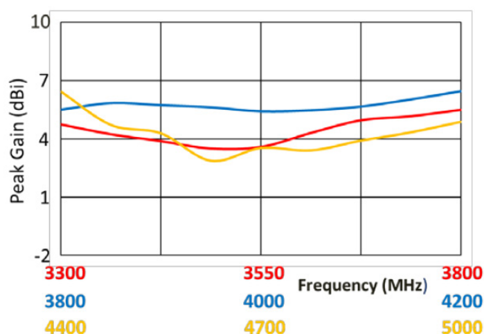
Peak Gain
