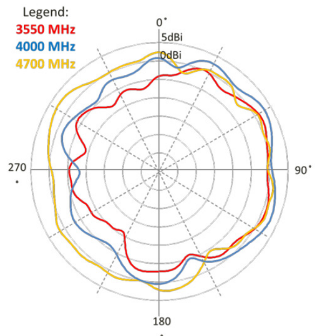
Elevation 2(YZ)
