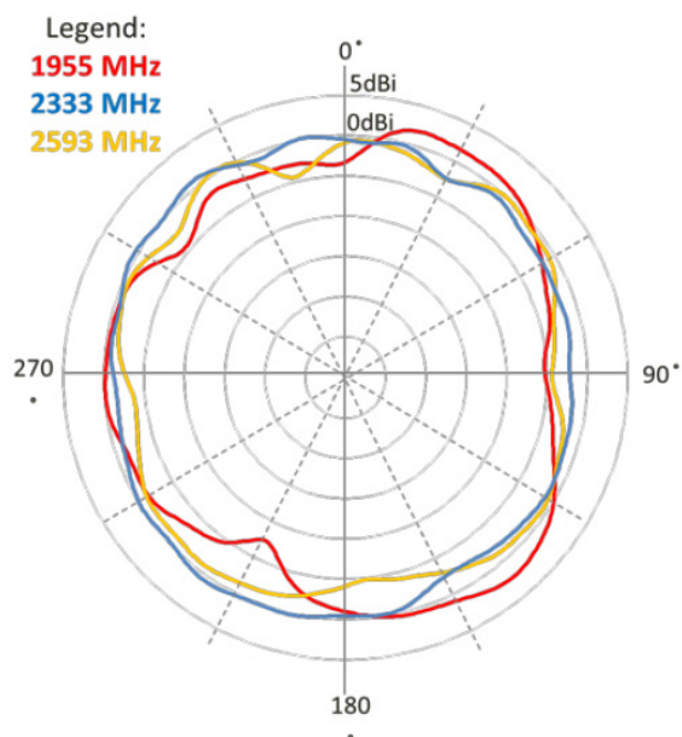
Elevation 2(YZ)
