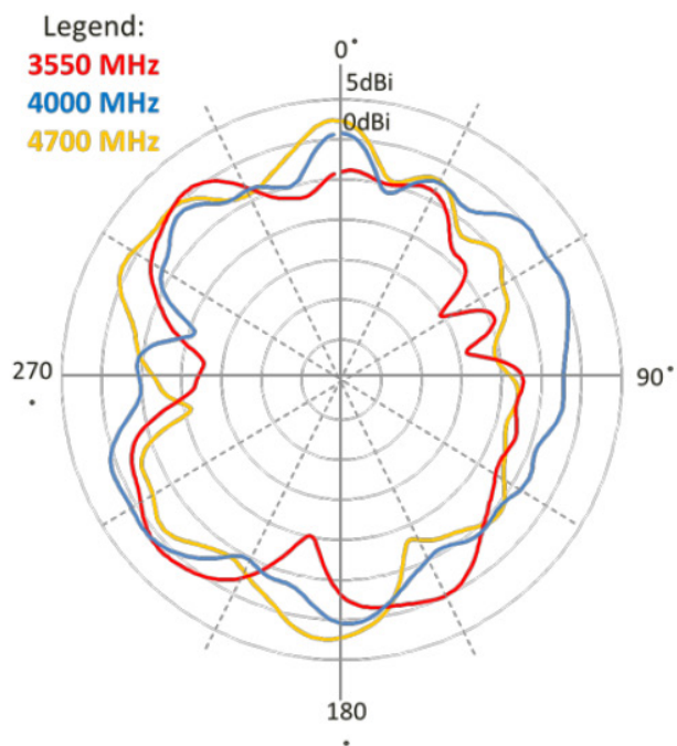
Elevation 1(XZ)
