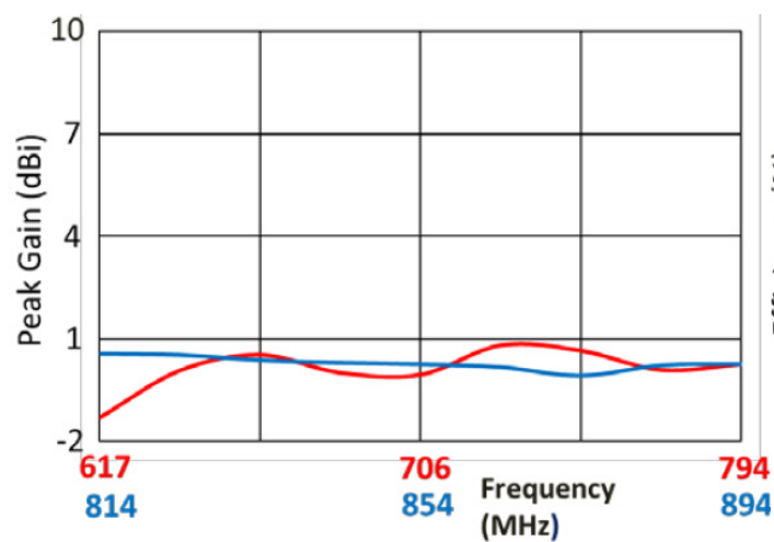
Peak Gain
