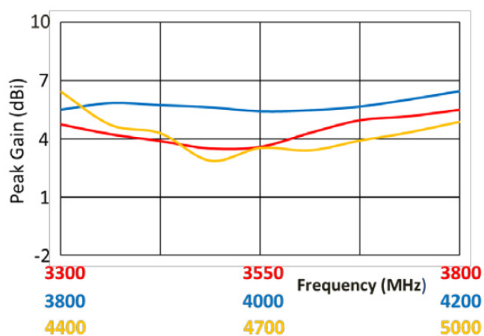
Peak Gain
