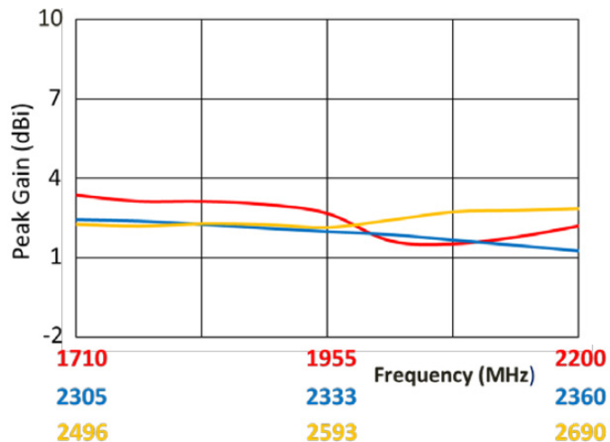
Peak Gain
