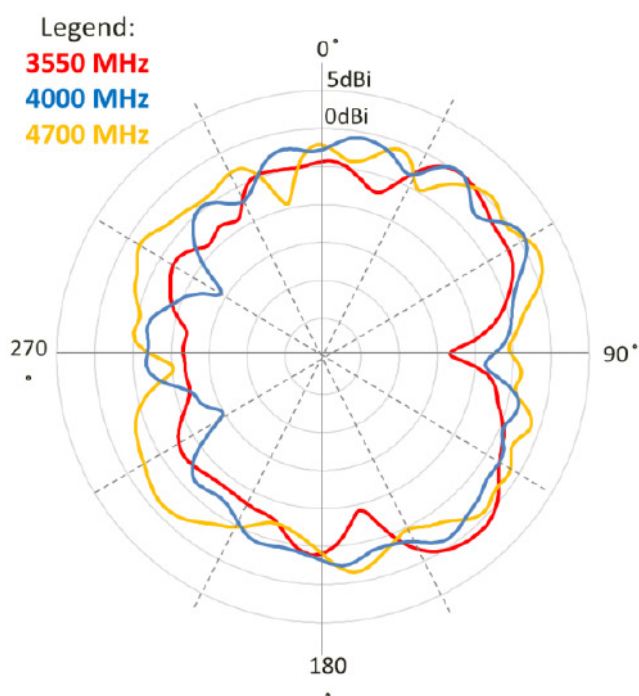
Elevation 2(YZ)
