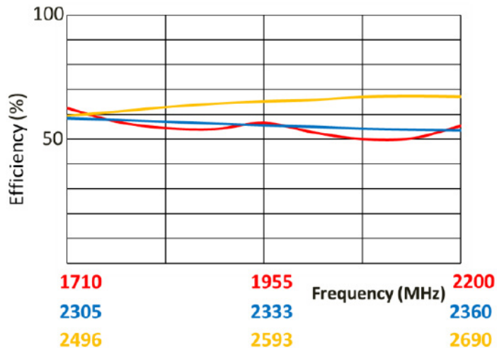
Efficiency
