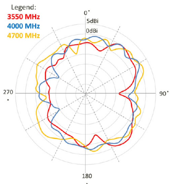
Elevation 2(YZ)
